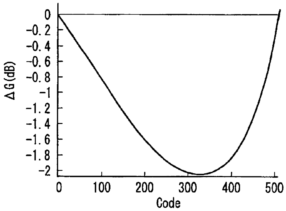
FIG. 10 PRIOR ART
