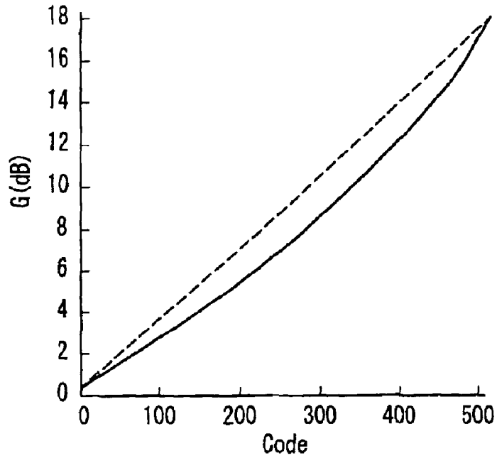
FIG. 8 PRIOR ART
