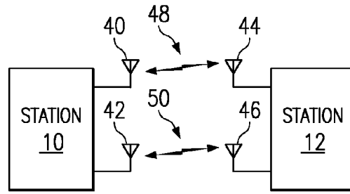
FIG. 3 (PRIOR ART)
