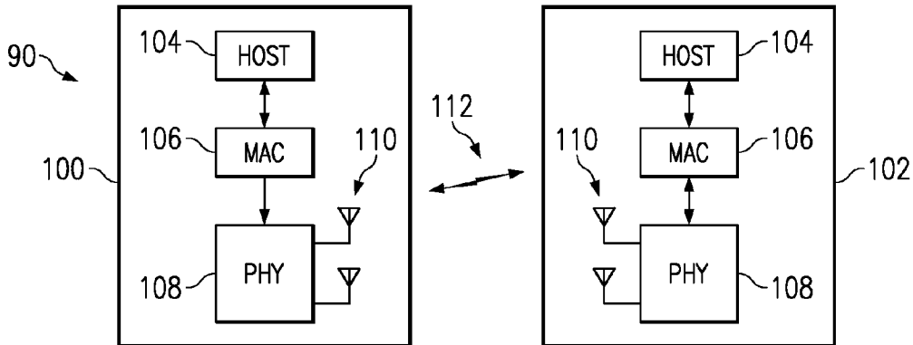
FIG. 5 (PRIOR ART)
