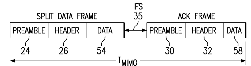
FIG. 4c (PRIOR ART)
