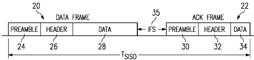
FIG. 2 (PRIOR ART)
