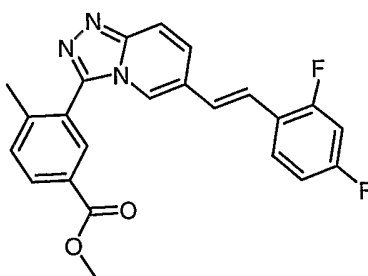
methyl 3-{6-[(E)-2-(2,4-difluorophenyl)vinyl][1,2,4]triazolo[4,3-a]pyridin-3-yl}-4-methylbenzoate
