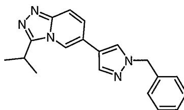
6-(1-benzyl-1H-pyrazol-4-yl)-3-isopropyl[1,2,4]triazolo[4,3-a]pyridine
