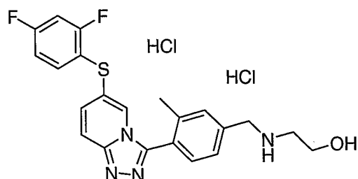
2-[(4-{6-[(2,4-difluorophenyl)thio][1,2,4]triazolo[4,3-a]pyridin-3-yl}-3-methylbenzyl)amino]ethanol dihydrochloride
