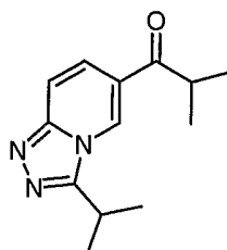
1-(3-isopropyl[1,2,4]triazolo[4,3-a]pyridin-6-yl)-2-methylpropan-1-one
