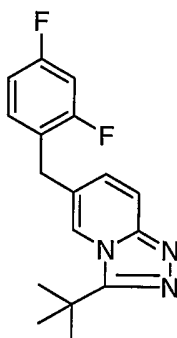
3-tert-butyl-6-(2,4-difluorobenzyl)[1,2,4]triazolo[4,3-a]pyridine
