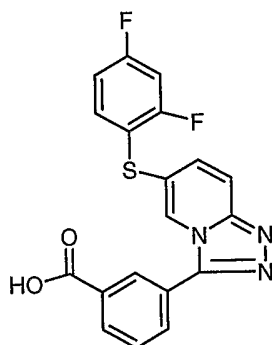
3-{6-[(2,4-difluorophenyl)thio][1,2,4]triazolo[4,3-a]pyridin-3-yl}benzoic acid
