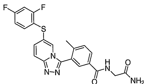
N-(3-{6-[(2,4-difluorophenyl)thio][1,2,4]triazolo[4,3-a]pyridin-3-yl}-4-methylbenzoyl)glycinamide
