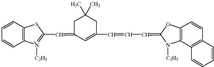
Sensitizing dye SD-2
