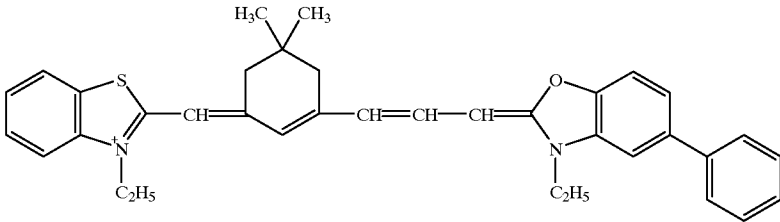
Sensitizing dye SD-3
