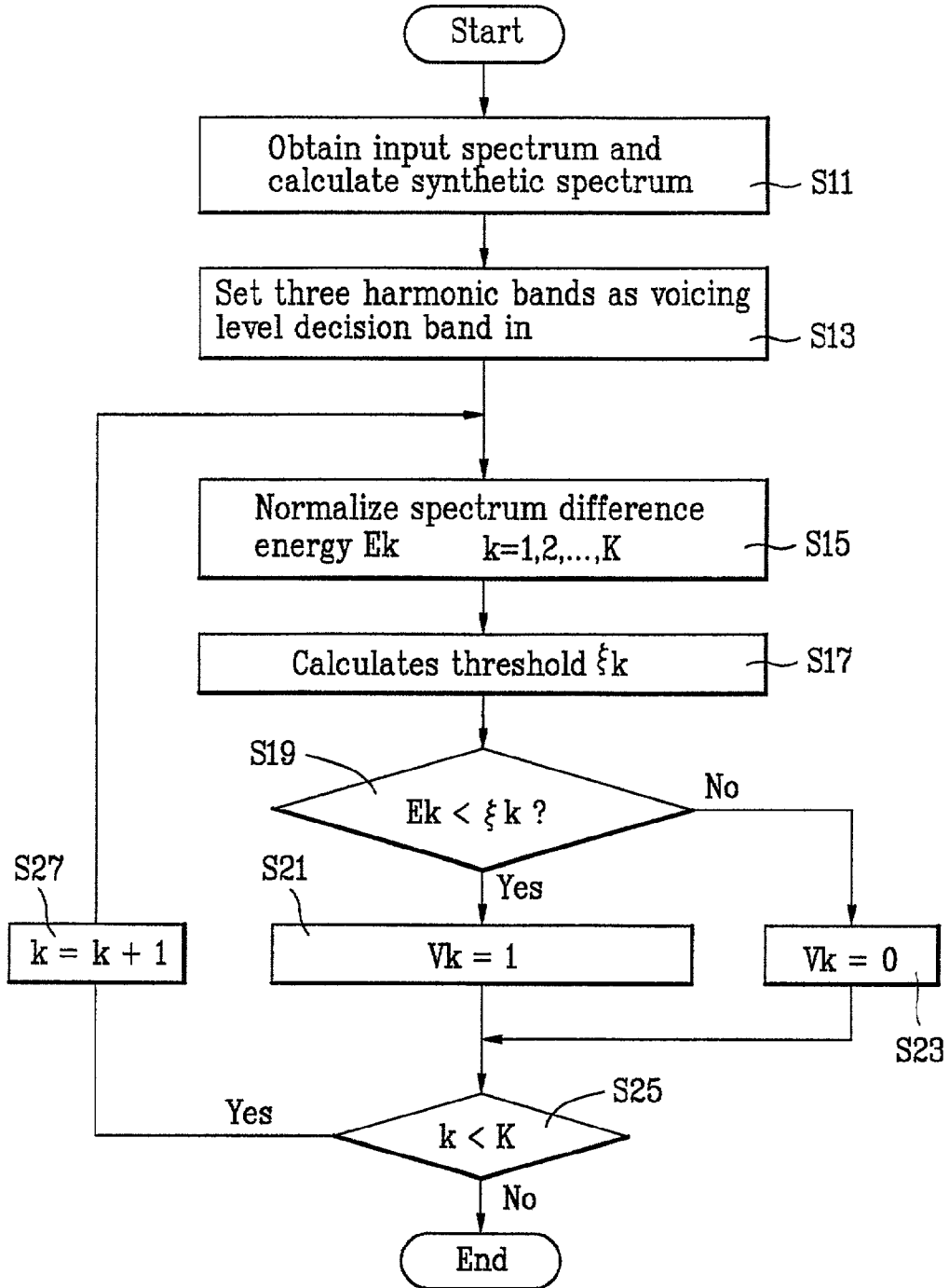
FIG. 2 Related Art
