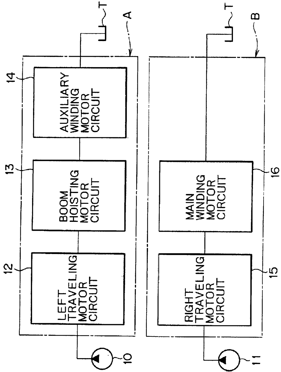
FIG. 5 PRIOR ART
