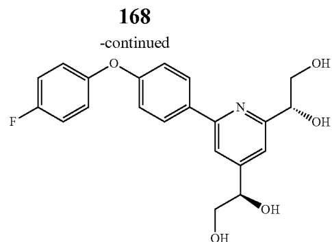
Compound Example No. 19
