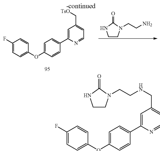
Compound Example No. 105
