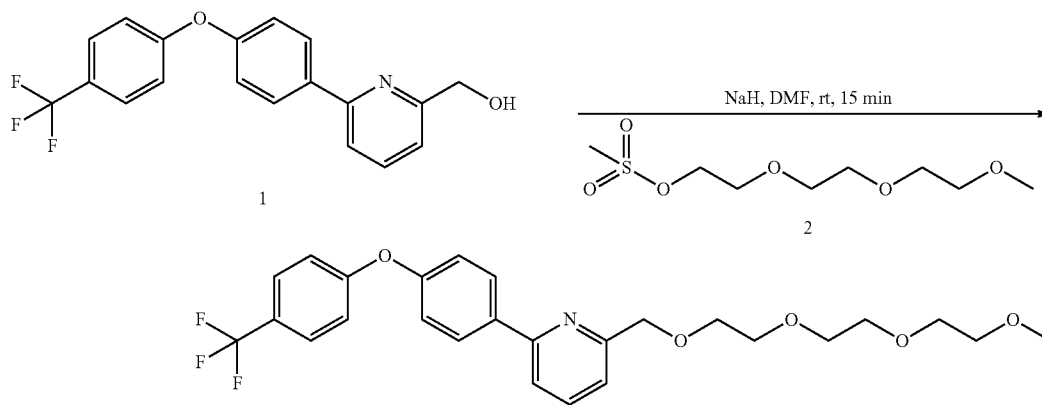
Compound Example No. 1
