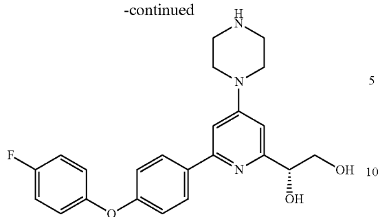
Compound Example No. 21
