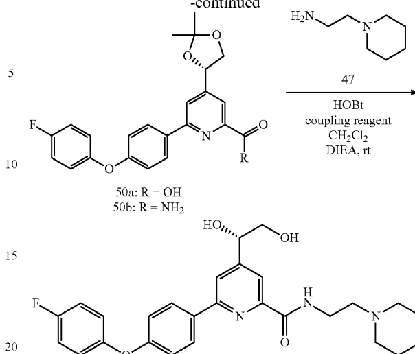
Compound Example No. 42
