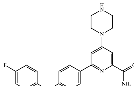
Compound Example No. 55
