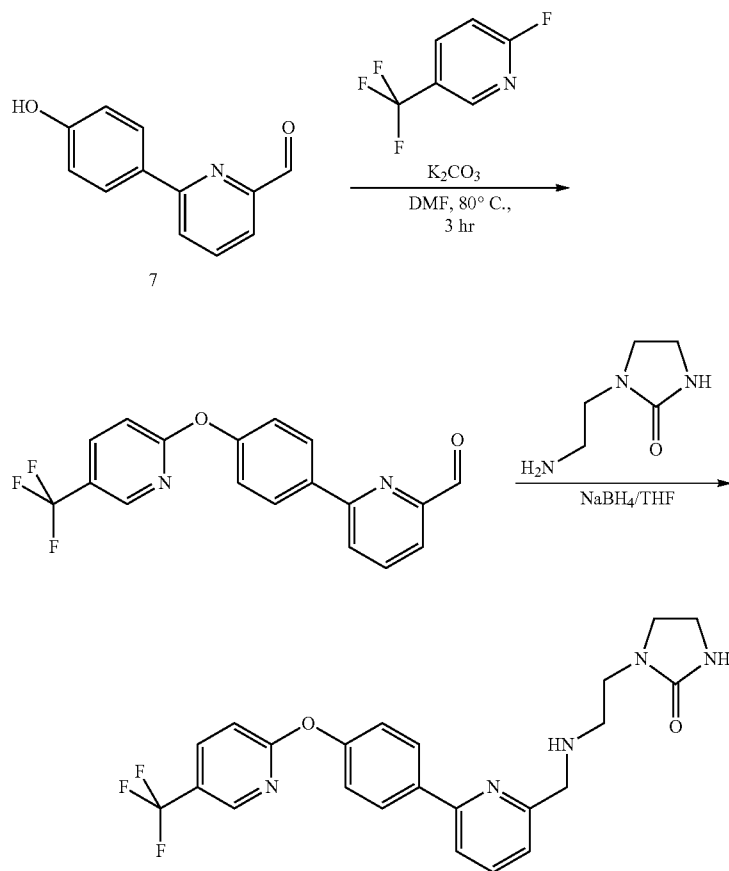
Compound Example No. 68
