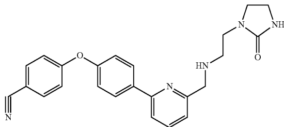
Compound Example No. 67
