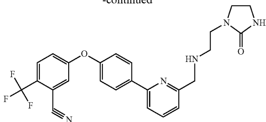
Compound Example No. 70
