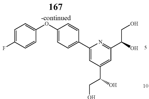
Compound Example No. 26
