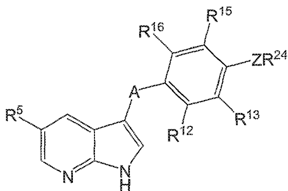
Formula IIIh
