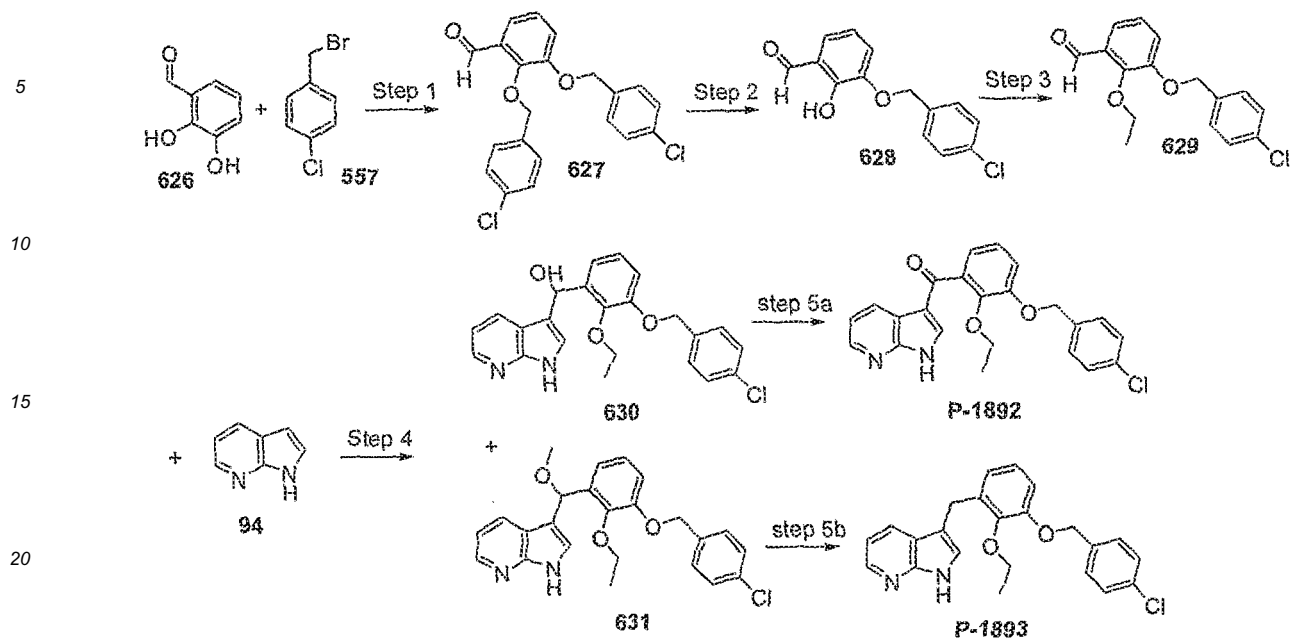
Scheme 71
