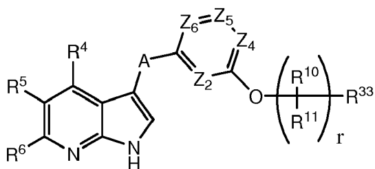
Formula IIId
