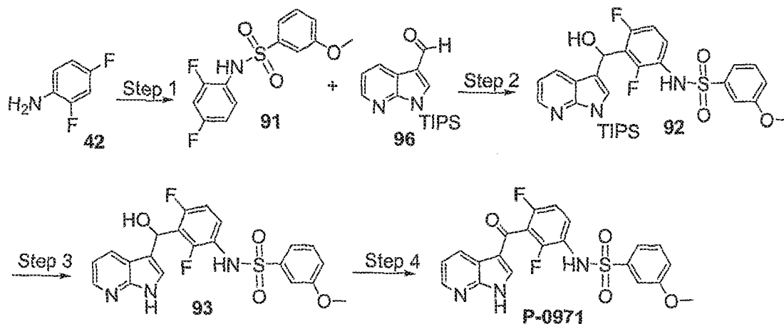
Scheme 26
