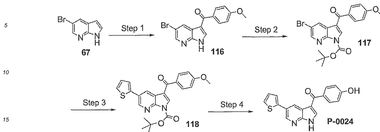
Scheme 35
