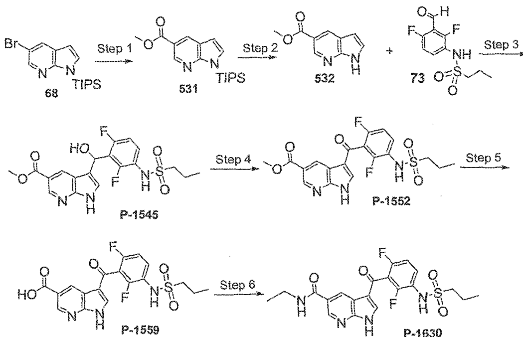
Scheme 45
