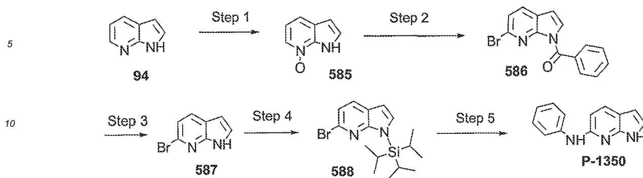
Scheme 40
