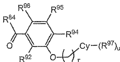
Formula VIb
