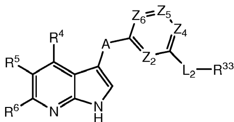
Formula IIIo
