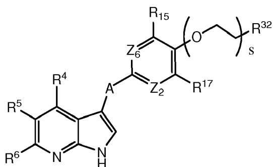
Formula IIIc
