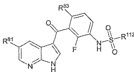
Formula IIIIm
