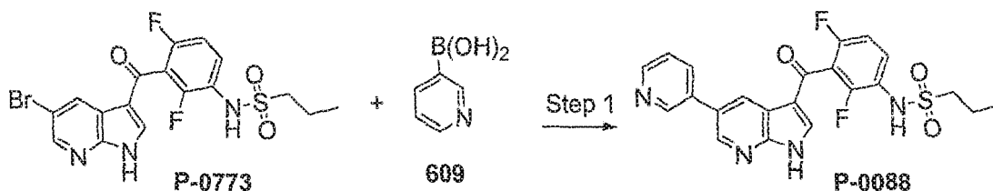
Scheme 15
