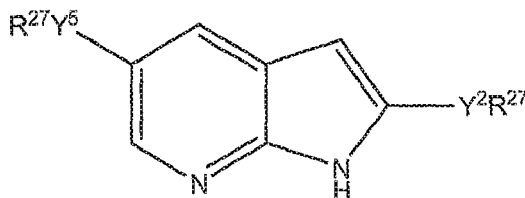
Formula If
