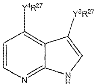
Formula Ib
