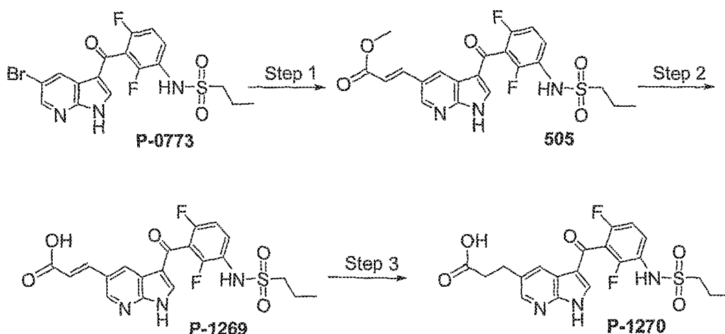
Scheme 38
