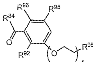
Formula IXa
