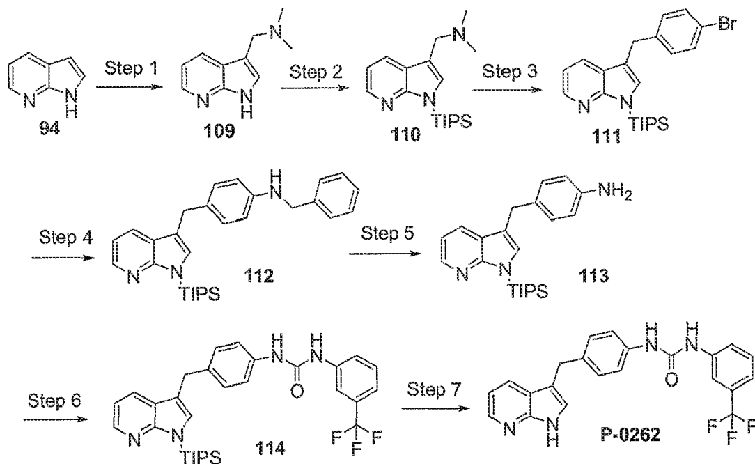
Scheme 34
