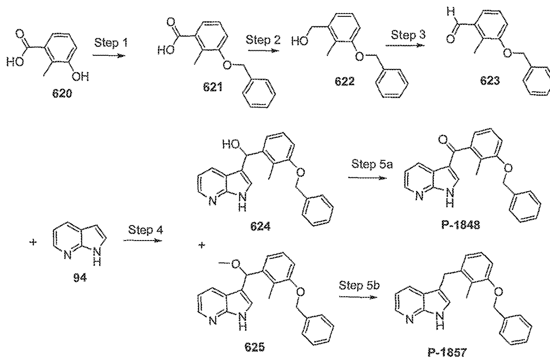
Scheme 70
