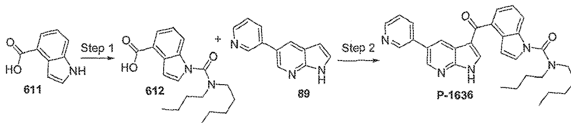
Scheme 68
