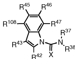
Formula VIII
