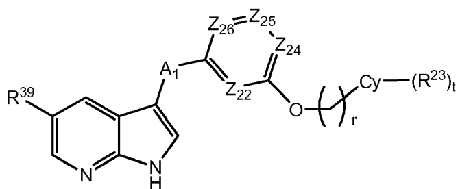
Formula IIIe
