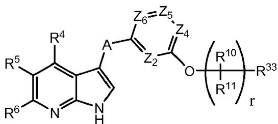
Formula IIId
