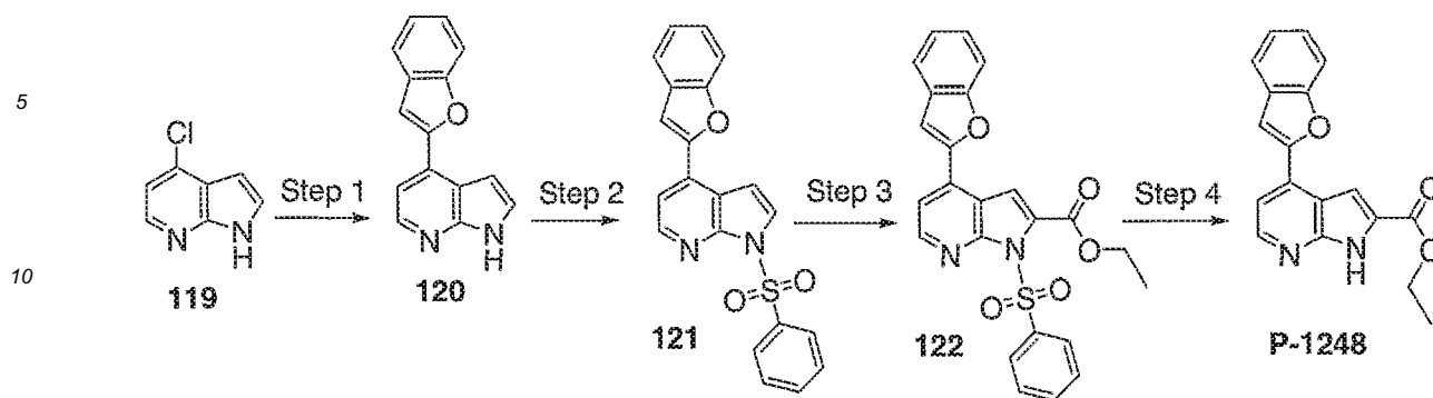
Scheme 36
