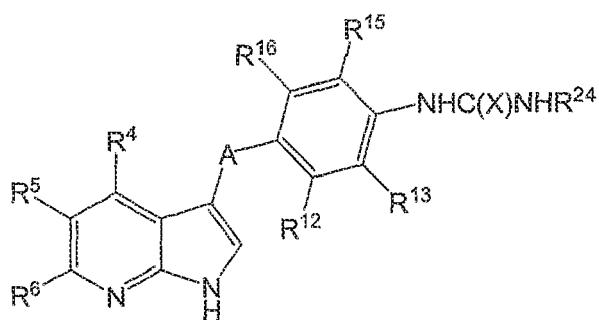
Formula IIj
