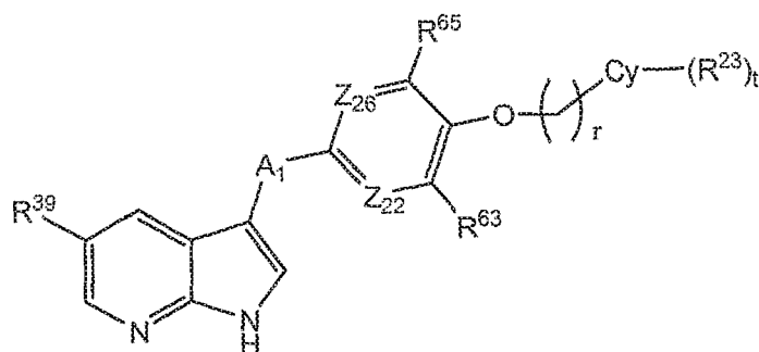
Formula IIIp
