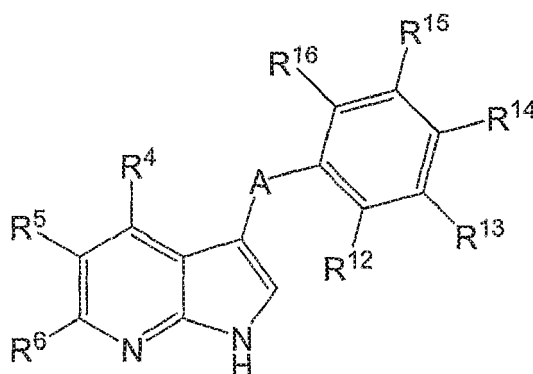
Formula II
