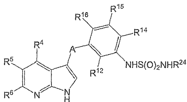
Formula IIg
