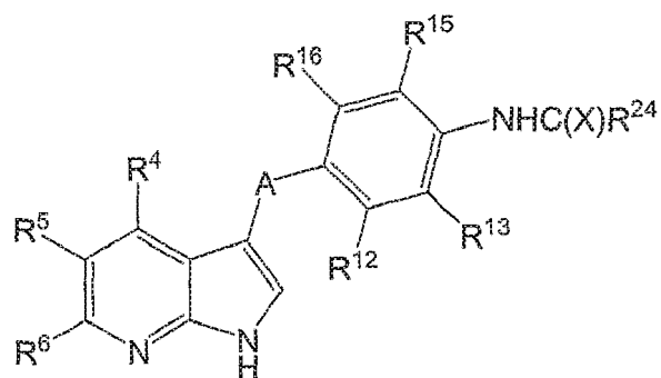
Formula IIIi
