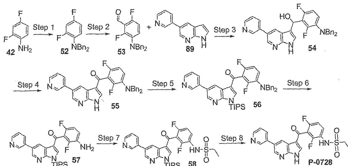
Scheme 16
