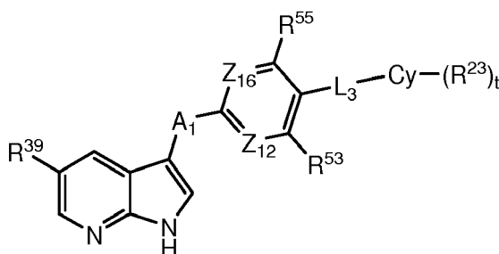
Formula IIIb
