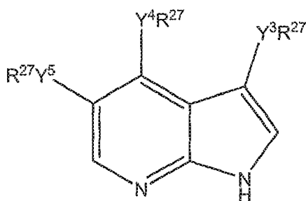
Formula Iw
