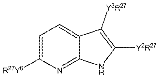
Formula Is
