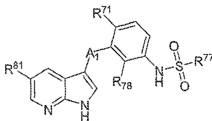
Formula IIIk
