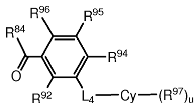
Formula VIa
