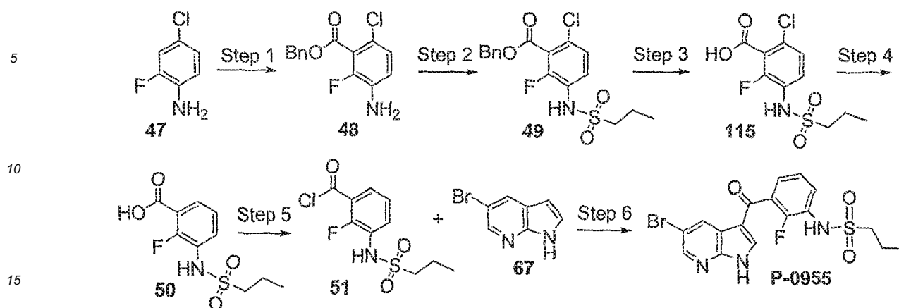
Scheme 14
