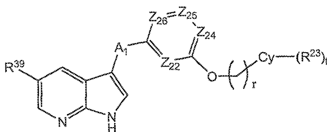
Formula IIIe
