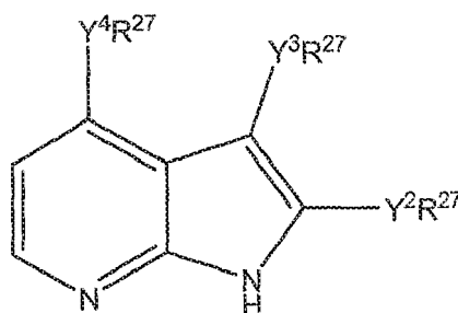
Formula Iq
