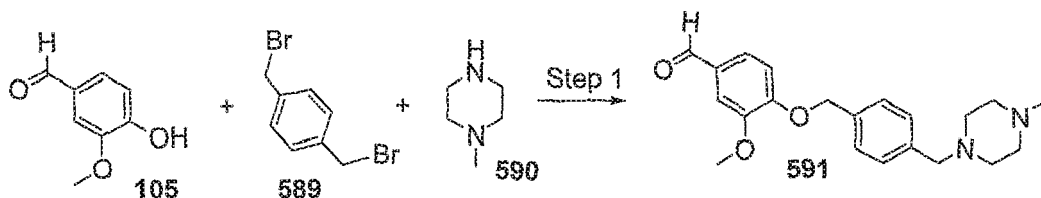
Scheme 59
