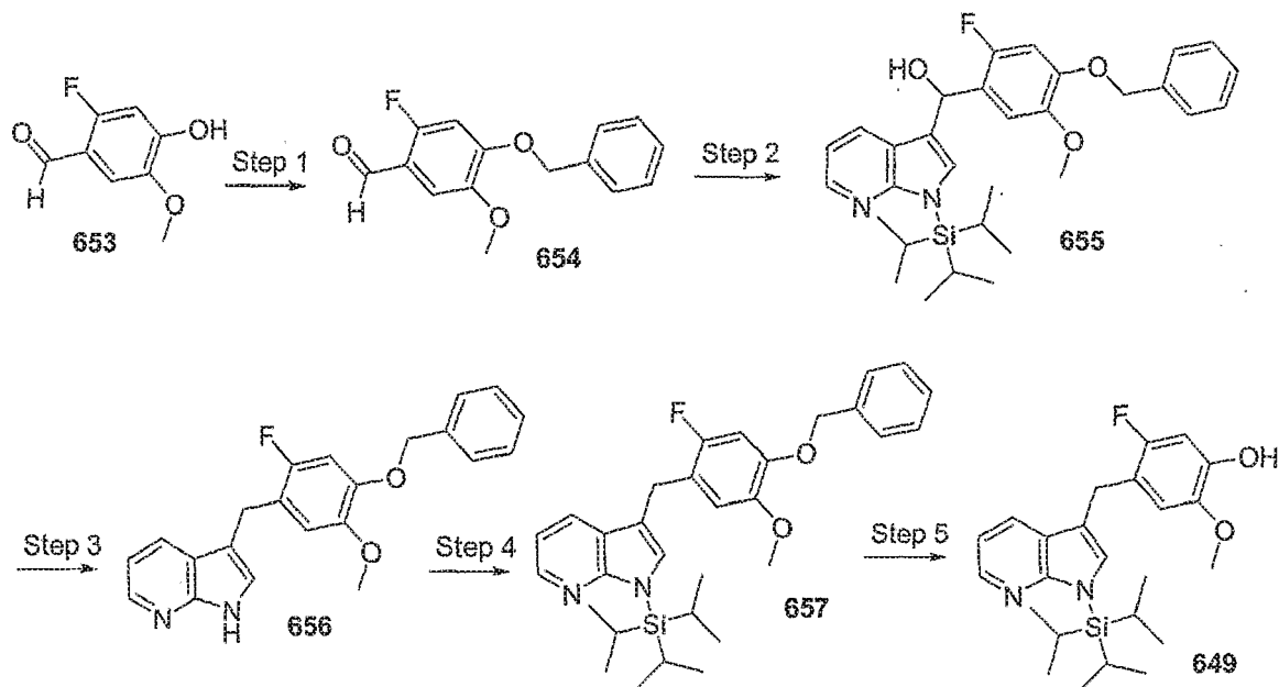
Scheme 80
