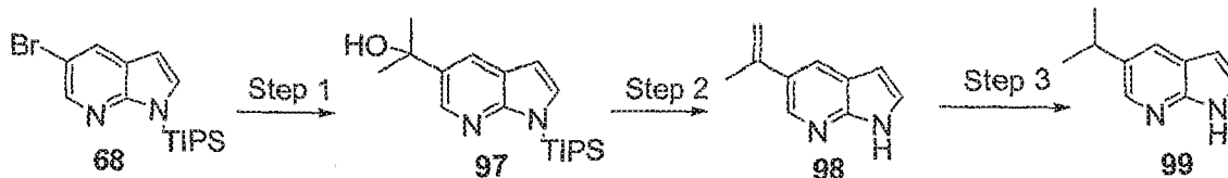
Scheme 28
