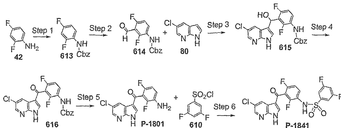
Scheme 67
