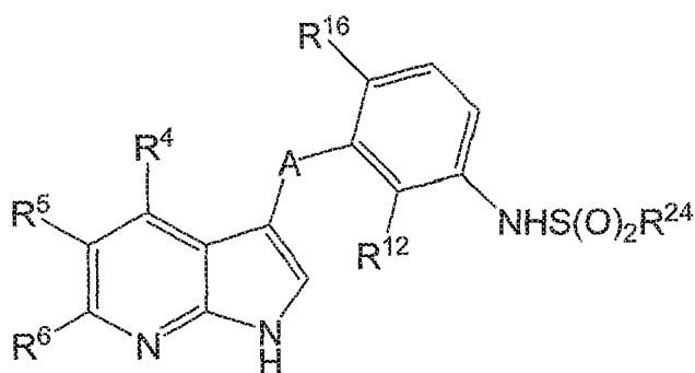
Formula IIa
