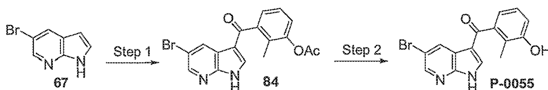
Scheme 22
