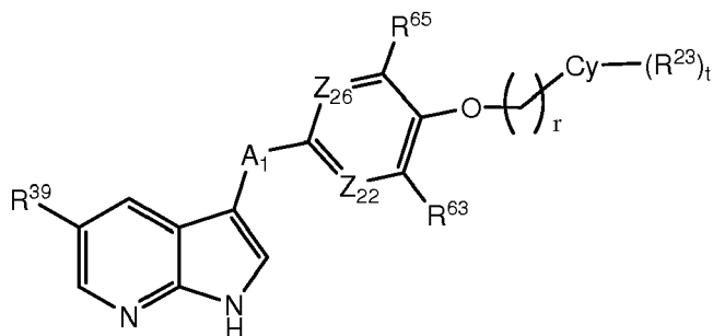
Formula IIIp
