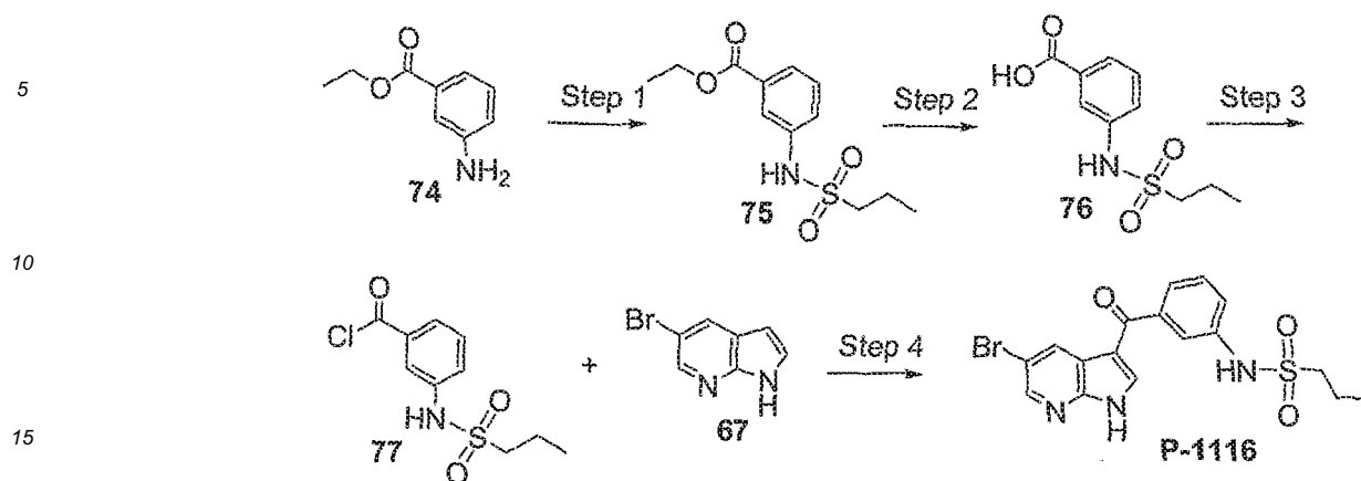
Scheme 20
