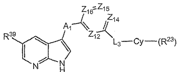
Formula IIIq
