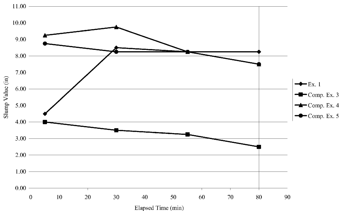
Concrete Slump Over Time
