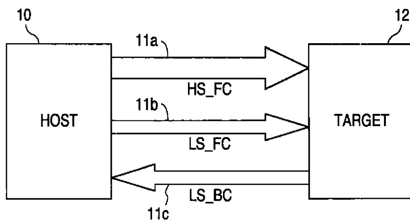
FIG. 1 (PRIOR ART)
