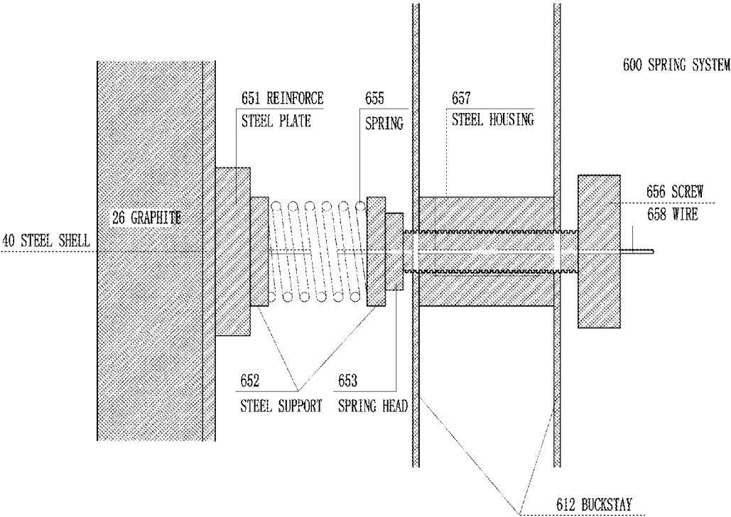
FIGURE 10 SIDE VIEW OF SPRING ARRANGMENT
