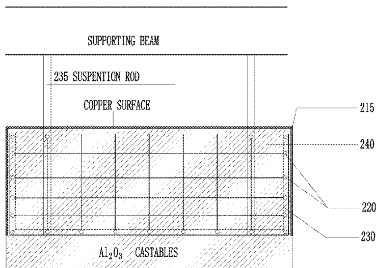
FIGURE 6 WATER COOLED BLOCK SECTION
