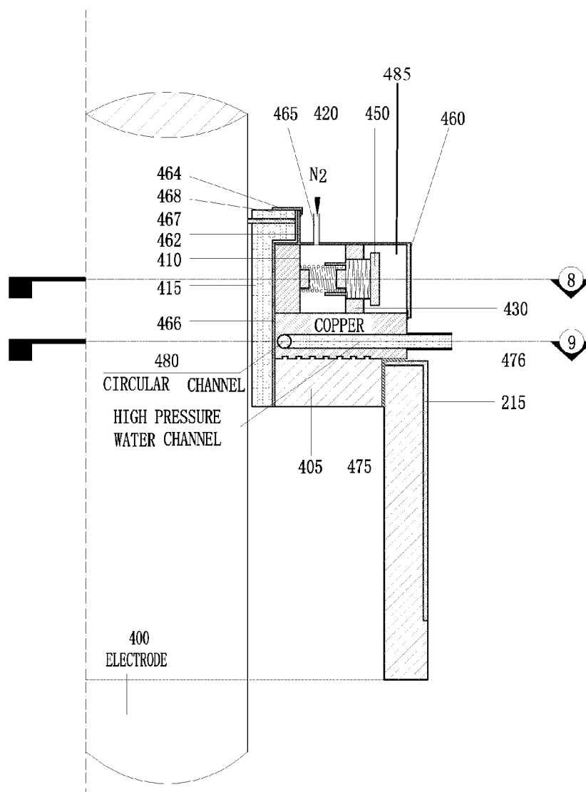
FIGURE 7 ELECTRODE SECTION
