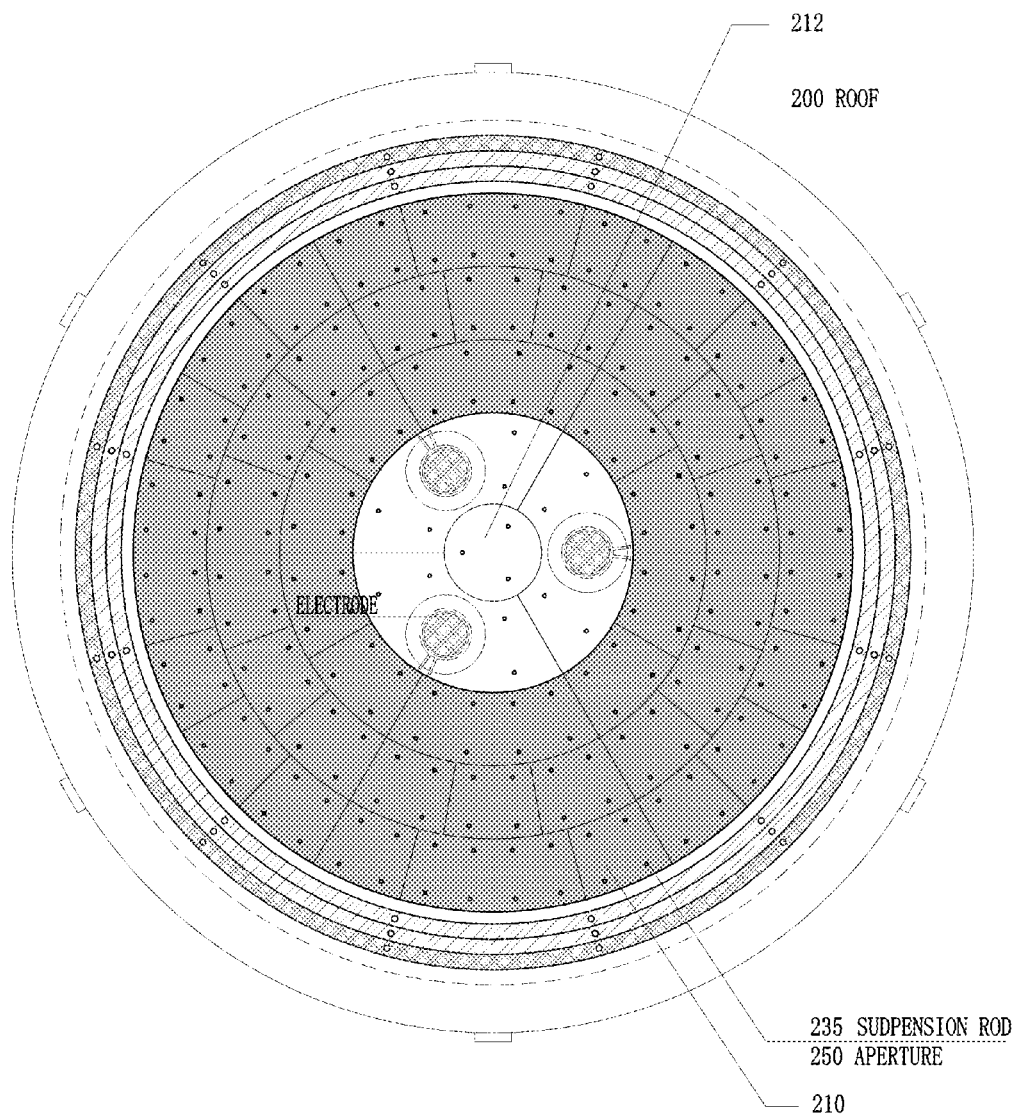
FIGURE 5 ELECTRIC FURNACE TOP PLAN
