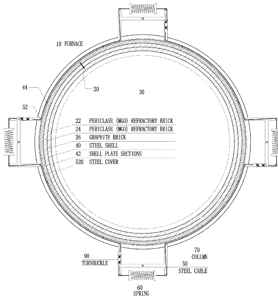
ELECTRIC FURNACE MIDDLE PLAN
