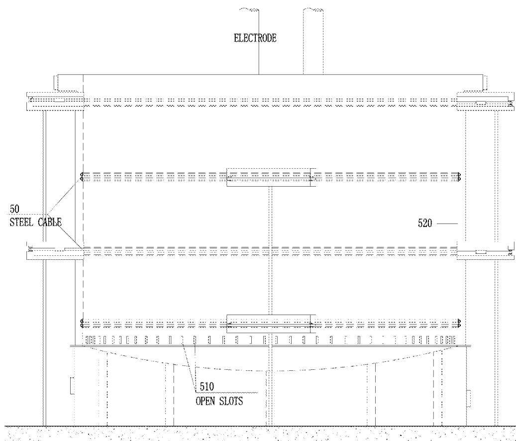
FIGURE 4 ELECTRICAL FURNACE ELEVATION
