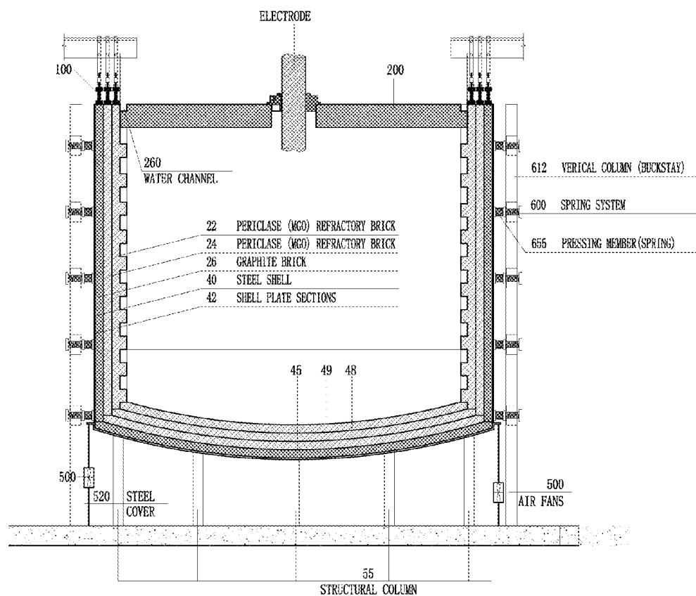
FIGURE 2 ELECTRIC FURNACE SECTION
