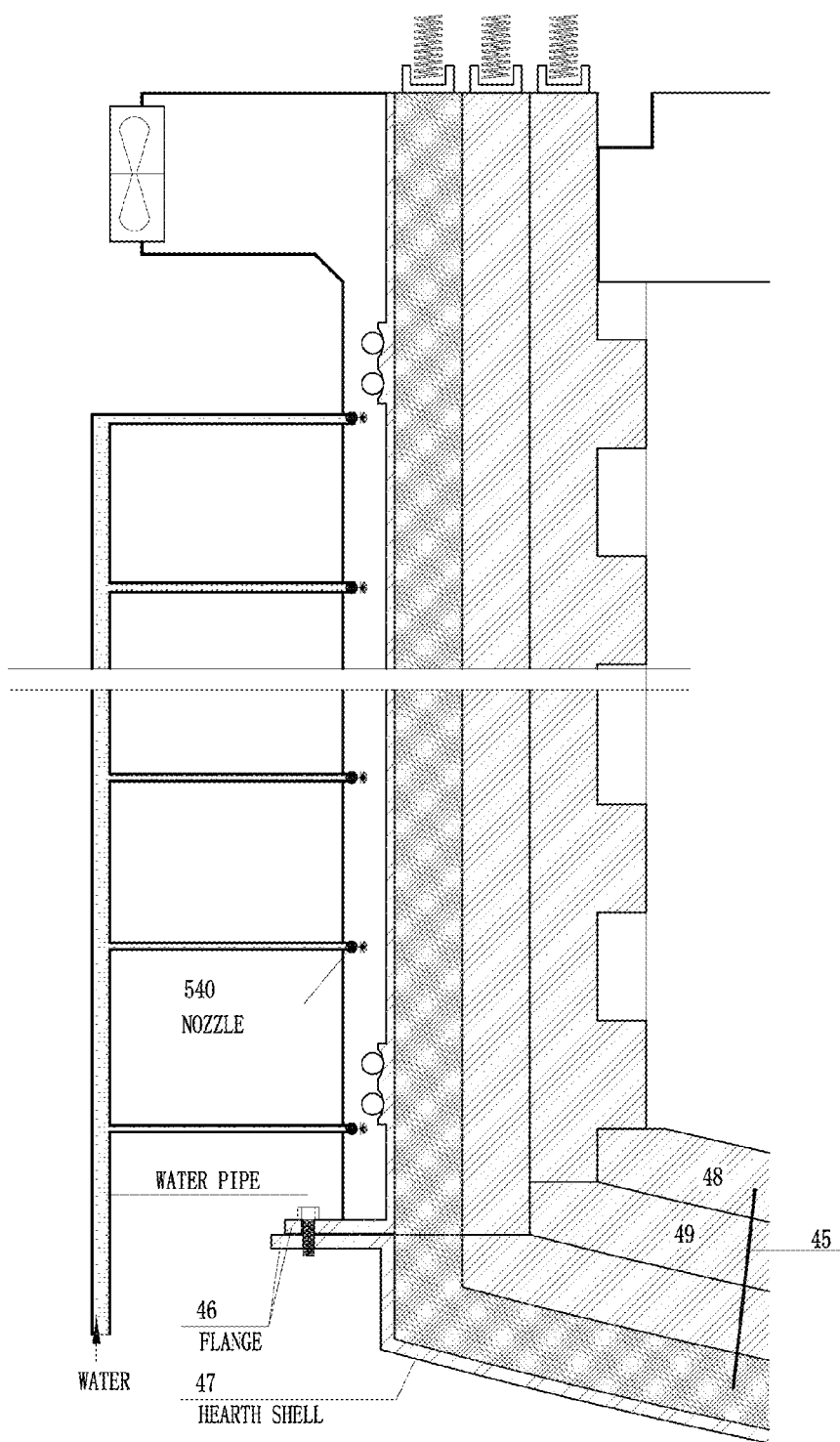
FIGURE 4A ELECTRICAL FURNACE DETAIL
