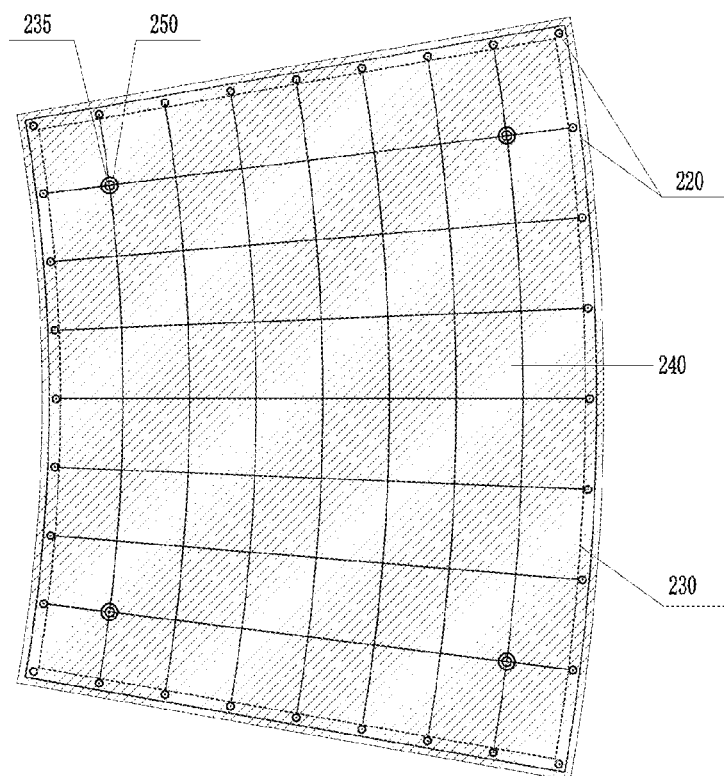
FIGURE 6A WATER COOLED BLOCK BOTTOM PLAN
