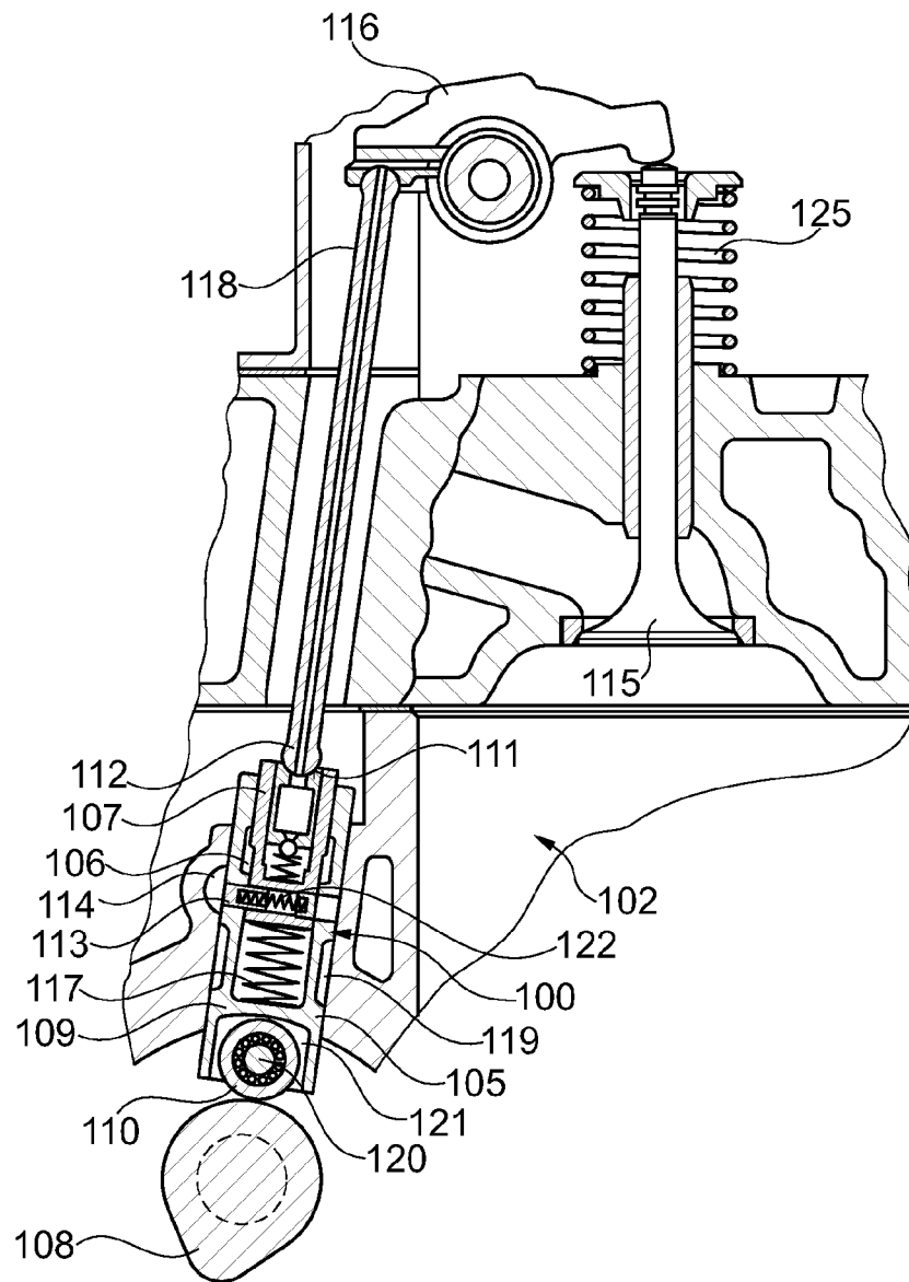
Fig. 8 PRIOR ART
