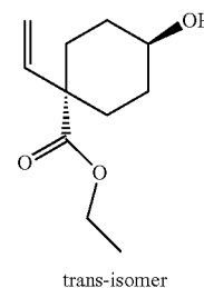
trans-isomer
