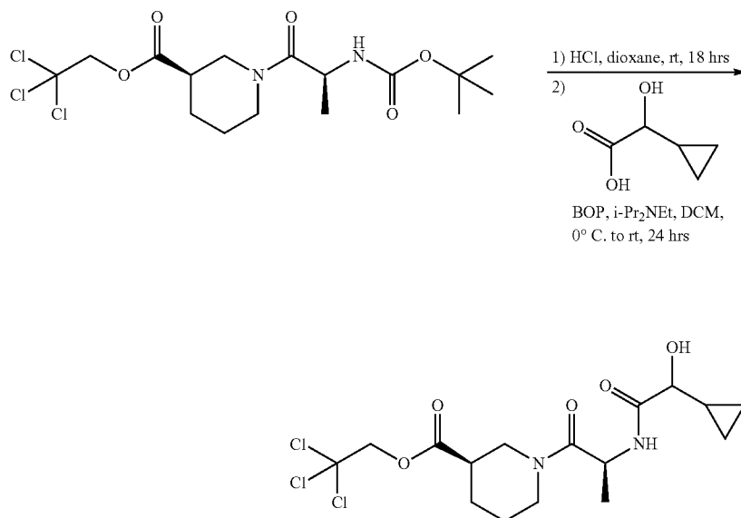
Compound 66a
