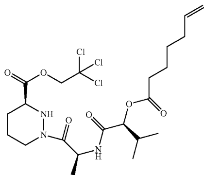
Compound 8a
