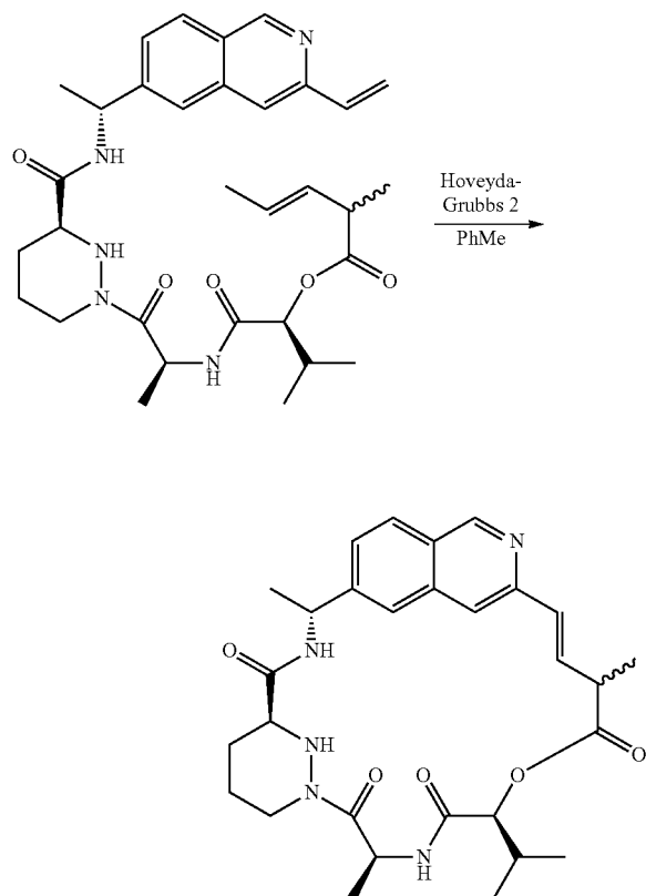
Compound 5
