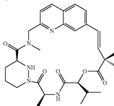
Compound 33
