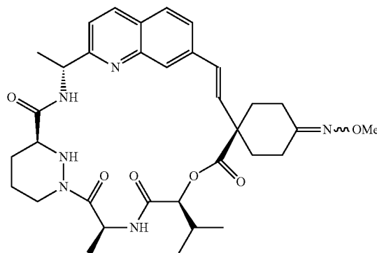
Compound 83
