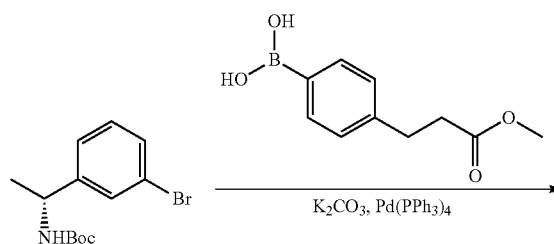
Compound 6b
