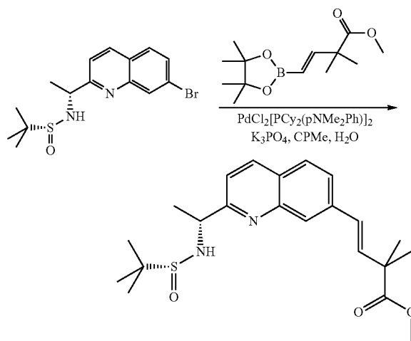
Compound 18d
