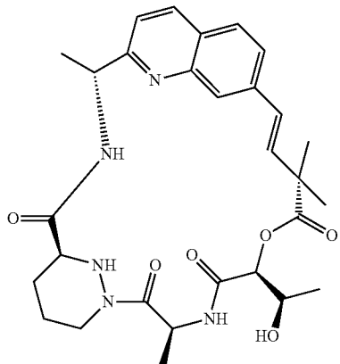
Compound 86a
