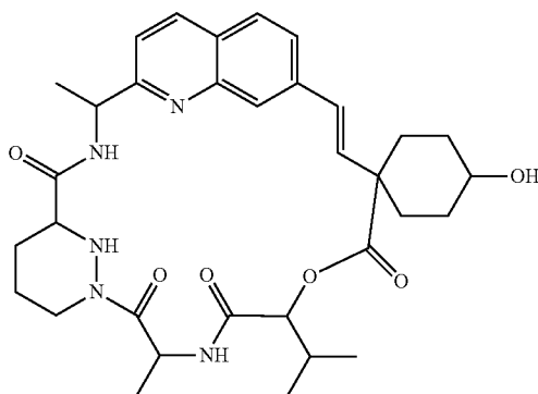
Compounds 76 and 77
