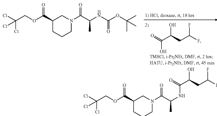
Compound 62e
