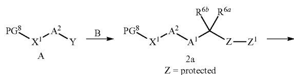
Scheme 4: Macrolactamization/Macrolactonization Connection 5
