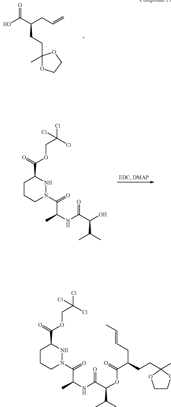
Compound 13b
