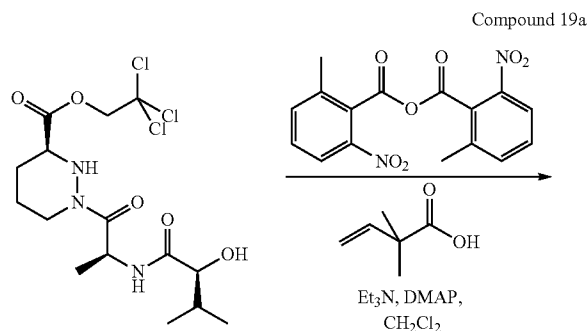
Compound 19a
