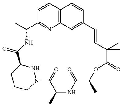
Compound 61
