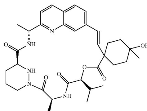
Compound 89a
