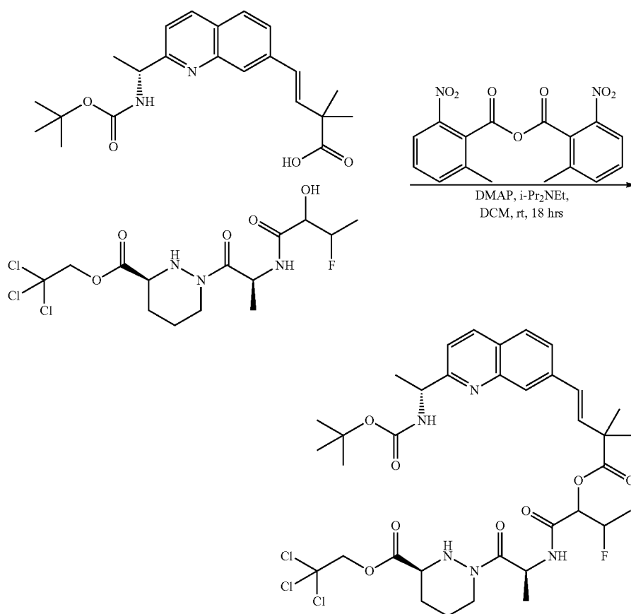
Compound 68c
