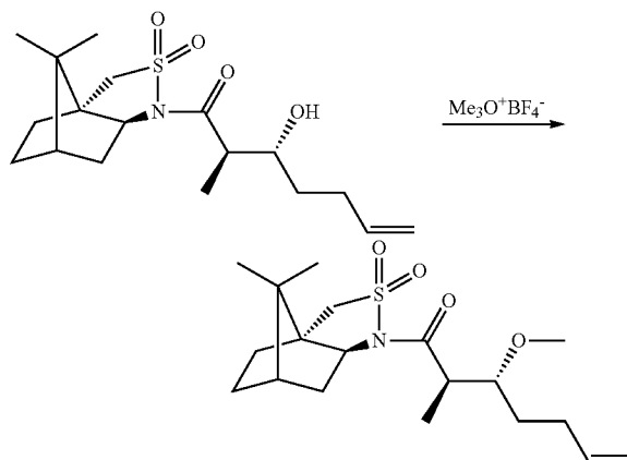
Compound 1b
