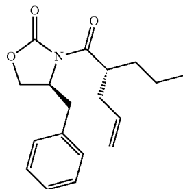
Compound 4b
