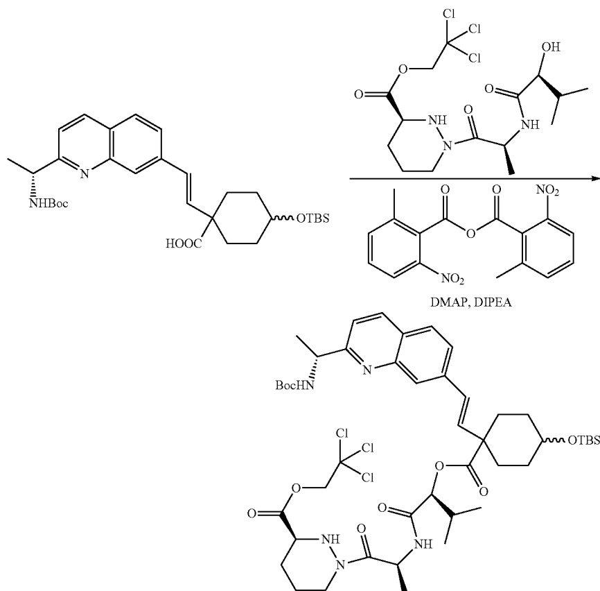
Compound 74d
