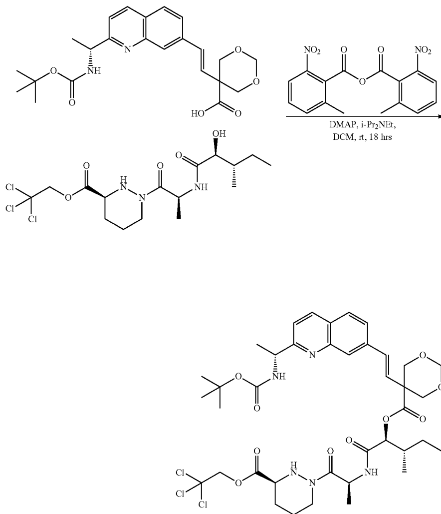
Compound 65c
