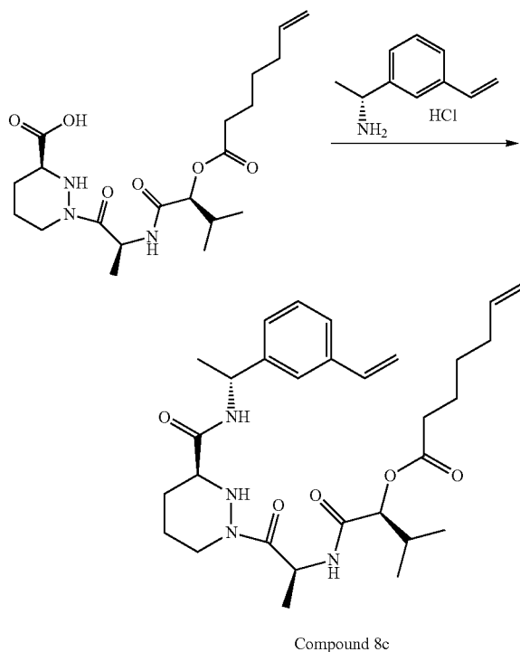
Compound 8c
