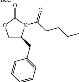
Compound 4a
