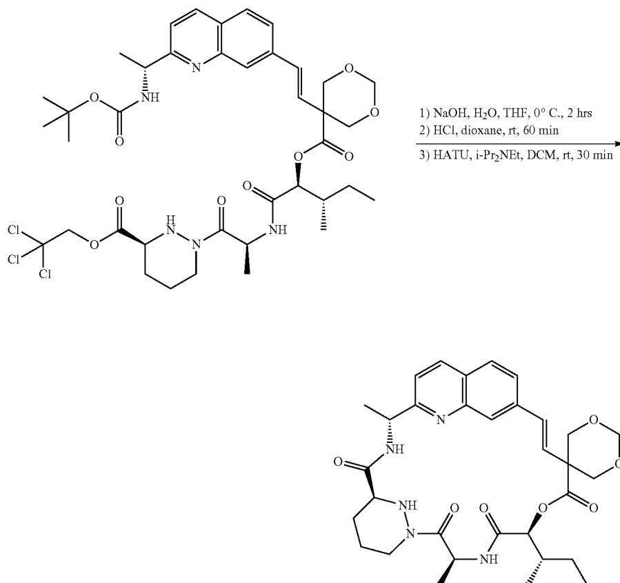
Compound 65
