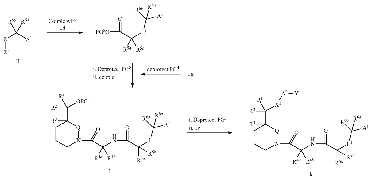
Scheme 3: RCM method
