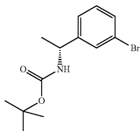
Compound 1h
