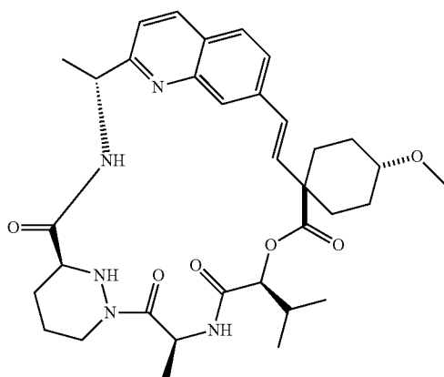
Compound 92a
