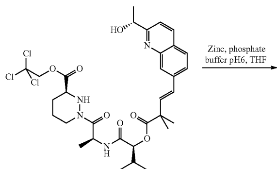
Compound 19c
