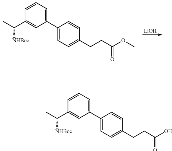
Compound 6c
