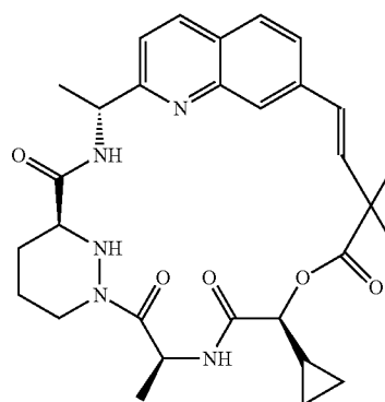
Compound 78a
