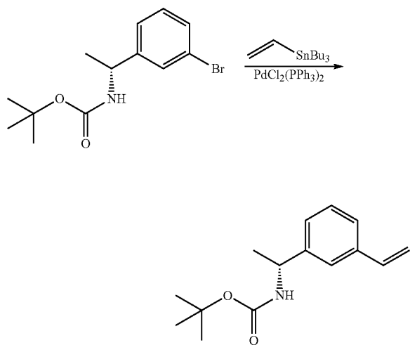
Compound 1i
