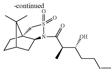
Compound 1a
