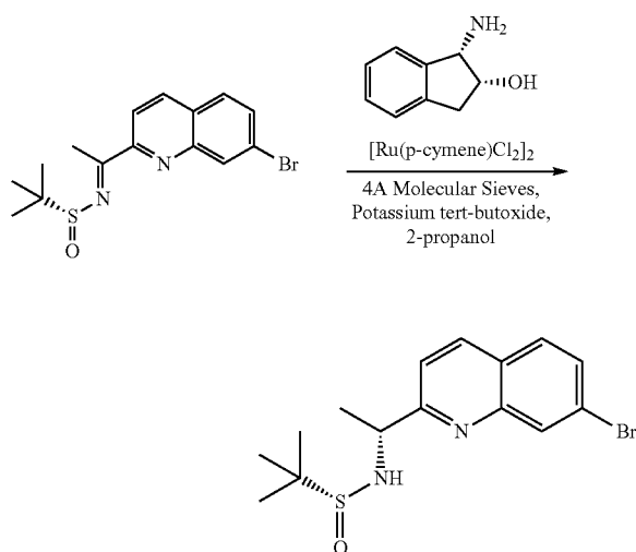
Compound 18c
