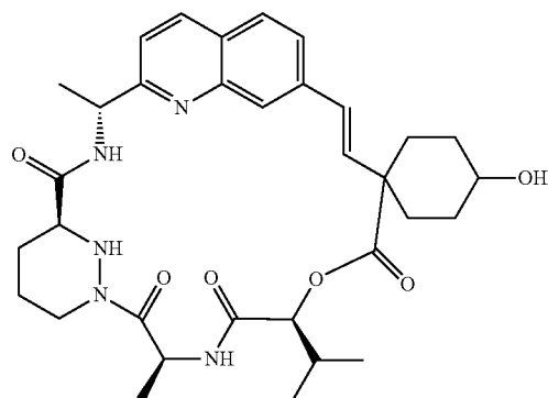
Compounds 74 and 75
