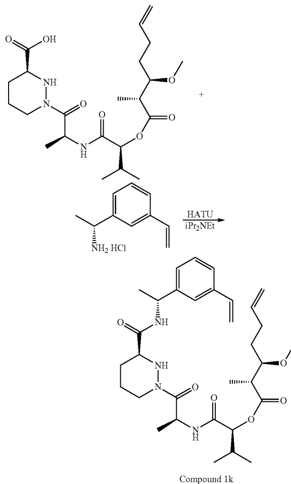
Compound 1k
