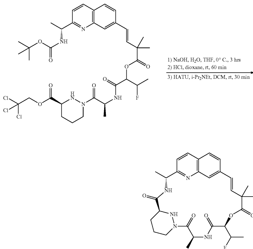
Compound 68
