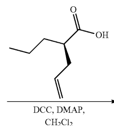
Compound 4d
