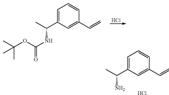
Compound 1j
