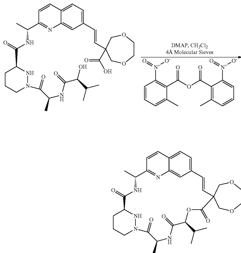
Compound 57
