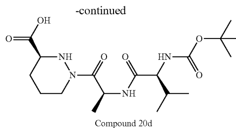
Compound 20d
