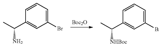
Compound 6a
