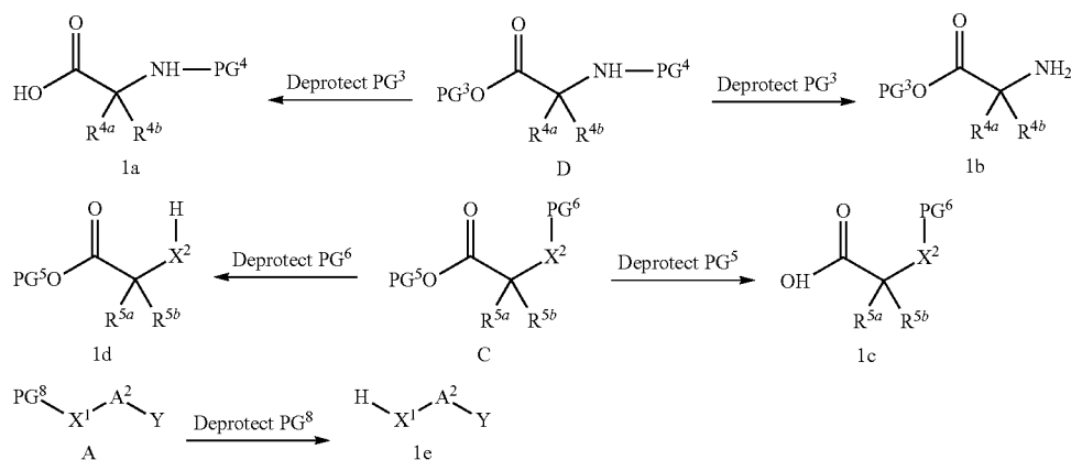
Scheme 2: RCM method
