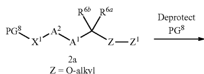
Scheme 5: Macrolactamization/Macrolactonization Connection 5
