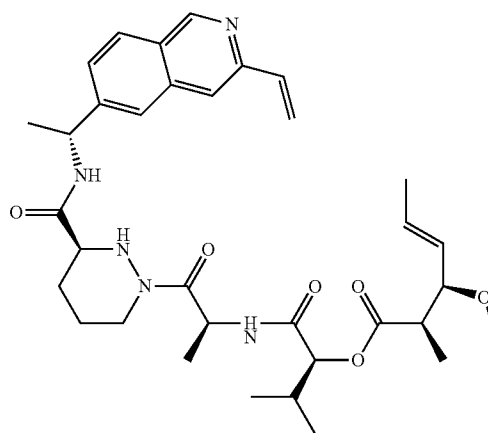
Compound 2k
