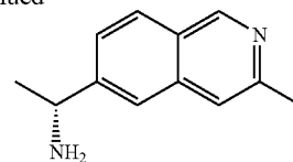
Compound 2j
