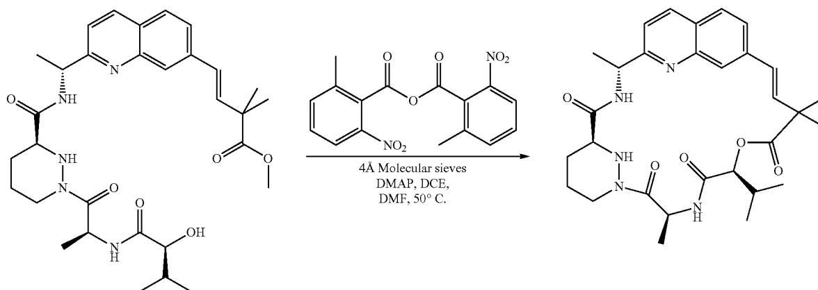
Compound 18
