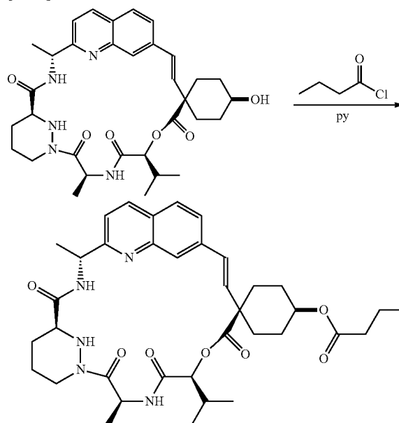
Compound 82
