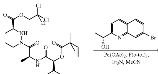
Compound 19b
