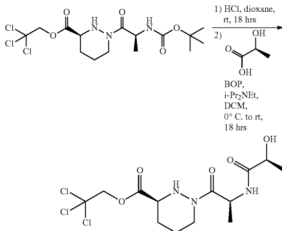
Compound 61a
