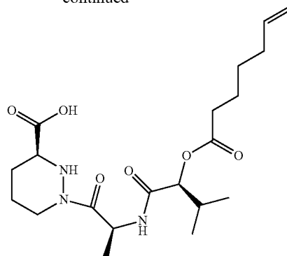
Compound 8b
