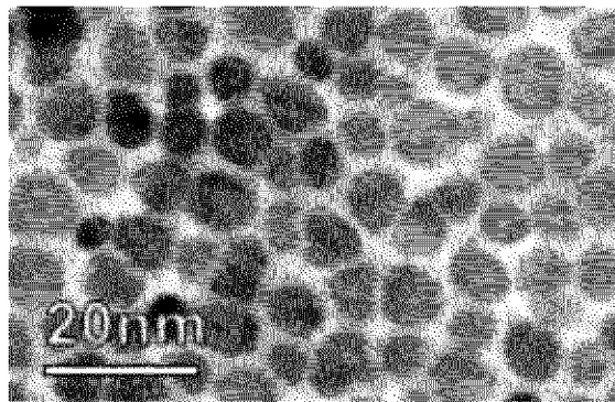
Co-Pt-Bi-TiO 2 -SiO 2
