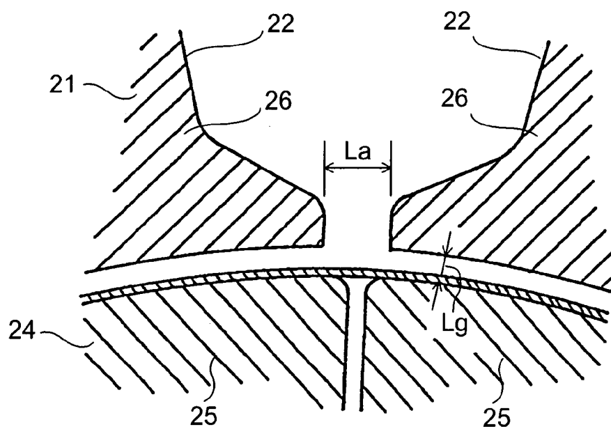
FIG. 19 PRIOR ART
