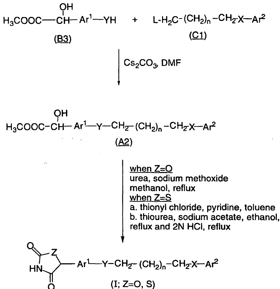
Scheme 3
