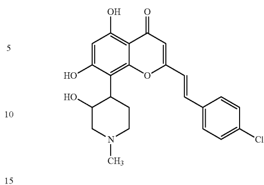
2-(4-Chlorostyryl)-5,7-dihydroxy-8-(3-hydroxy-1-methylpiperidin-4-yl)-4H-chromen-4-one; 32
