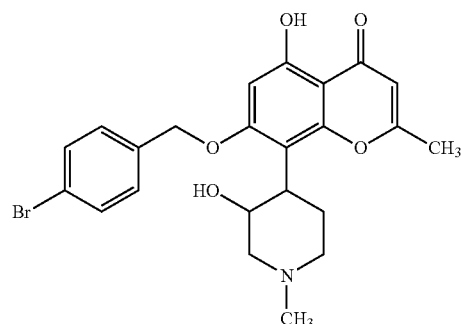
7-(4-Bromobenzyloxy)-5-hydroxy-8-(3-hydroxy-1-methylpiperidin-4-yl)-2-methyl-4H-chromen-4-one; 4
