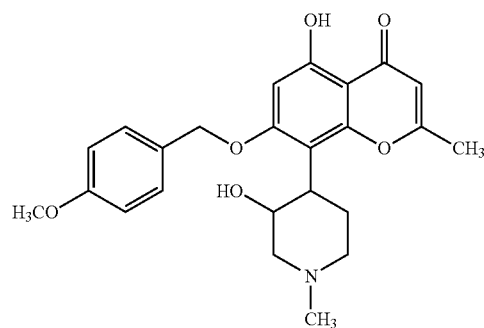
7-(4-Methoxybenzyloxy)-5-hydroxy-8-(3-hydroxy-1-methylpiperidin-4-yl)-2-methyl-4H-chromen-4-one; 3
