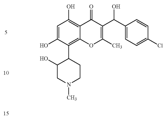
3-((4-Chlorophenyl)(hydroxy)methyl)-5,7-dihydroxy-8-(3-hydroxy-1-methylpiperidin-4-yl)-2-methyl-4H-chromen-4-one; 14
