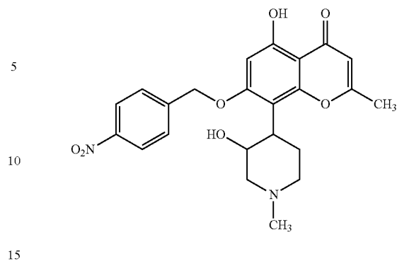
7-(4-Nitrobenzyloxy)-5-hydroxy-8-(3-hydroxy-1-methylpiperidin-4-yl)-2-methyl-4H-chromen-4-one; 8
