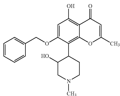
7-(Benzyloxy)-5-hydroxy-8-(3-hydroxy-1-methylpiperidin-4-yl)-2-methyl-4H-2
