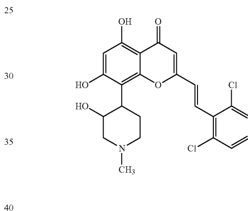
2-(2,3,4,5,6-Pentafluorostyryl)-5,7-dihydroxy-8-(3-hydroxy-1-methylpiperidin-4-yl)-4H-chromen-4-one; 33
