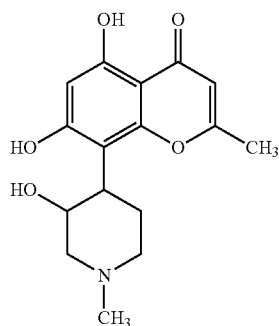
Rohitukine (1)
