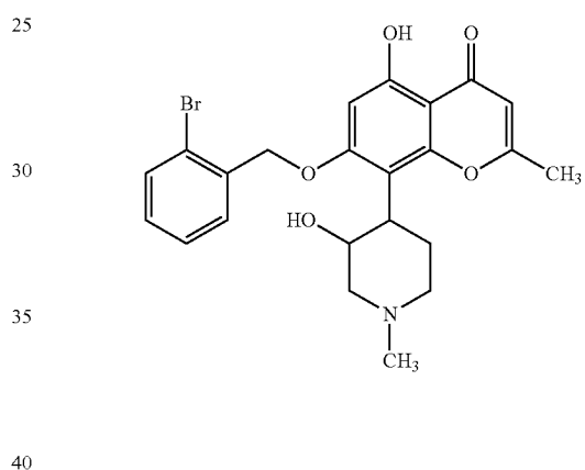
7-(2-Bromobenzyloxy)-5-hydroxy-8-(3-hydroxy-1-methylpiperidin-4-yl)-2-methyl-4H-chromen-4-one; 9
