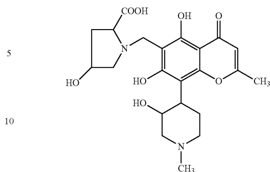
4-hydroxy-1-((5,7-dihydroxy-8-(3-hydroxy-1-methylpiperidin-4-yl)-2-methyl-4-oxo-4H-chromen-6-yl)methyl)pyrrolidine-2-carboxylic acid; 42
