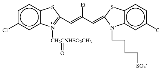
Sensitizing dye 8
