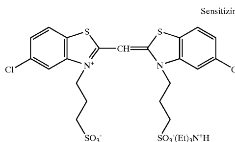
Sensitizing dye 1
