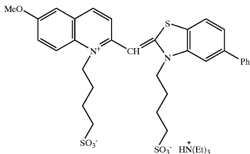
Sensitizing dye 3
