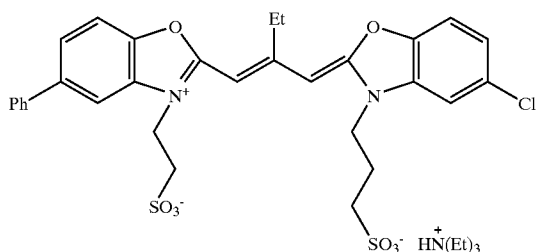
Sensitizing dye 4
