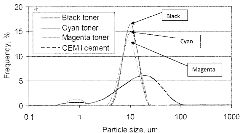
Figure 1. Particle size distribution of toners and Portland cement
