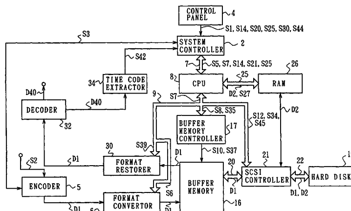
1 RECORDING/REPRODUCING APPARATUS
