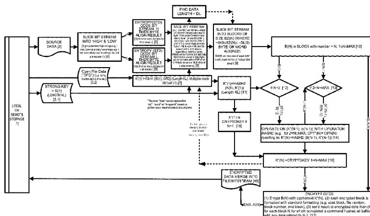
Figure 1: Bit Stream Sliced into Entropy Bands, Multiplexed and Block-Sliced and Encrypted in a Process Based on any Entropy and Encryption Coding Standards
