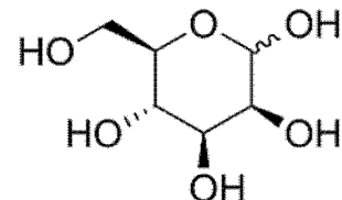
D-mannose
