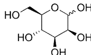
D-mannose
