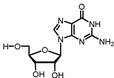
guanosine
