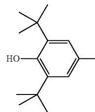
Butylated hydroxytoluene (BHT)
