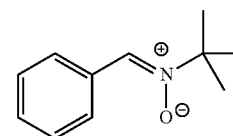
2-Phenyl-N-tert-butyl nitron (PBN)
