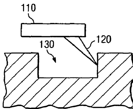
WIDE TRENCH
