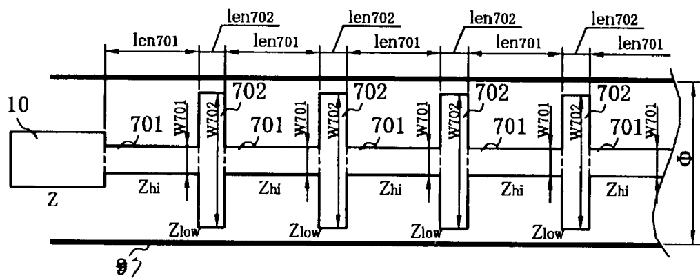
FIG. 7 PRIOR ART
