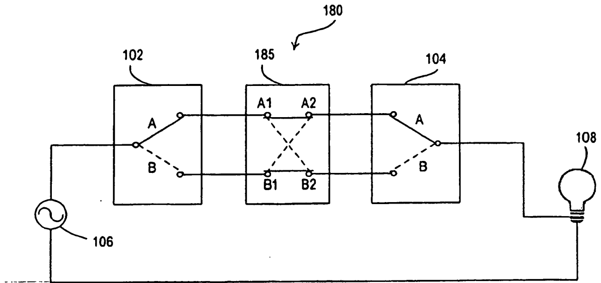
Fig. 1C Prior Art
