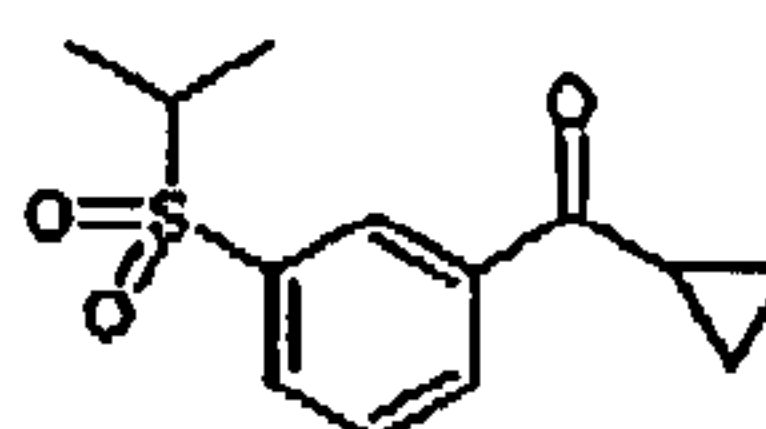
Intermediate az
