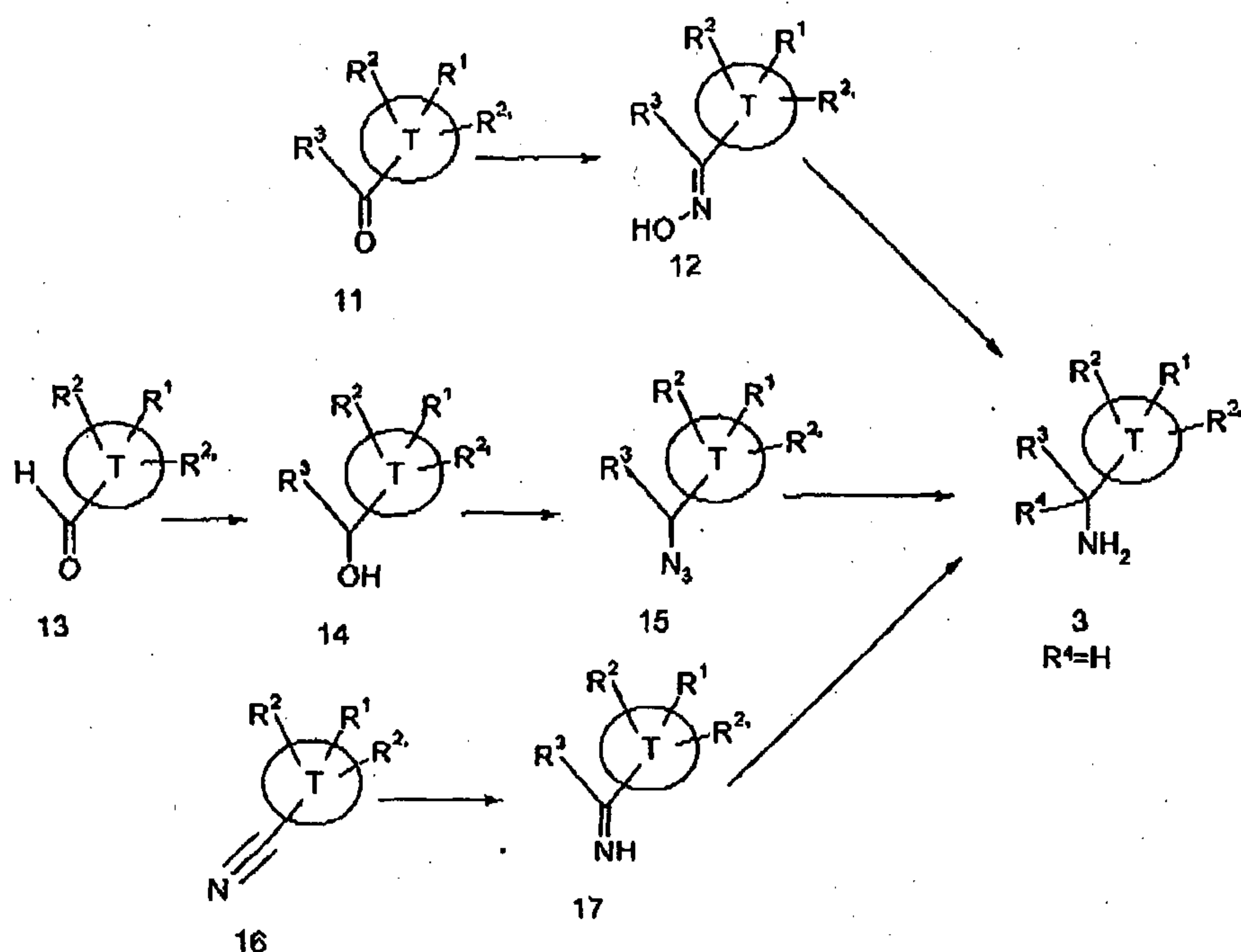
Scheme 5.
