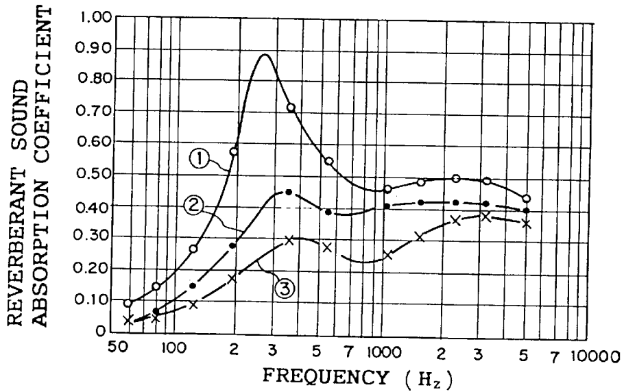
FIG. 48 (PRIOR ART)
