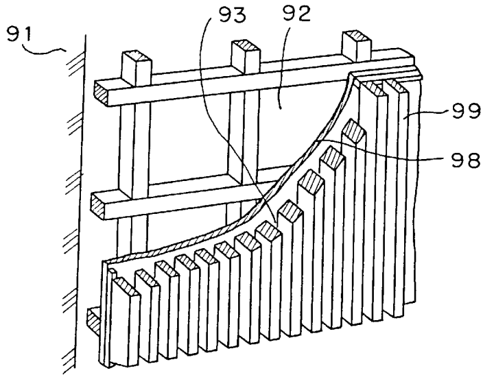
FIG. 47 (PRIOR ART)
