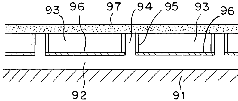
FIG. 45 (PRIOR ART)
