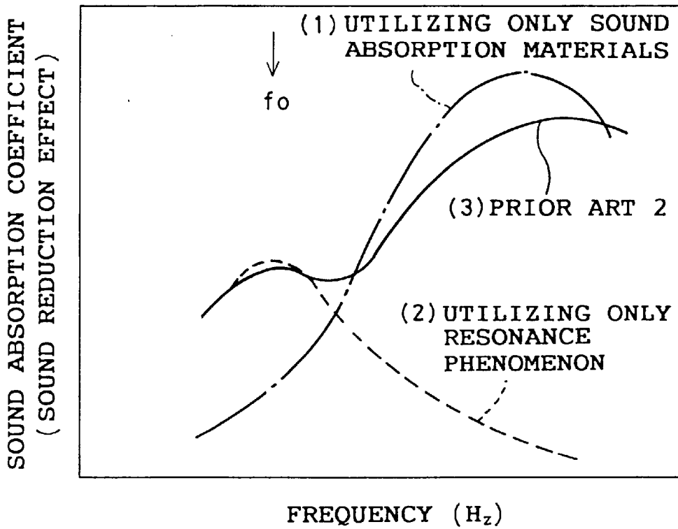
FIG. 46 (PRIOR ART)
