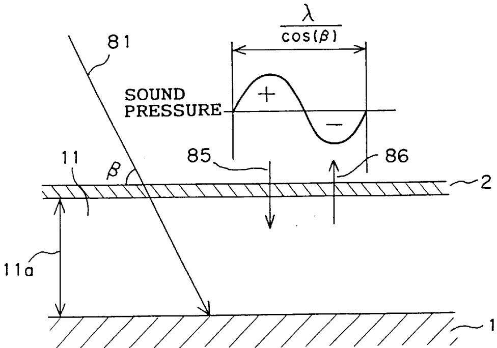
FIG. 44 (PRIOR ART)
