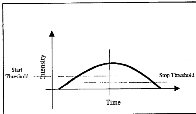
Location of the Peak
