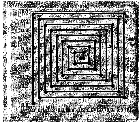
Spiral-like line-based scanning
