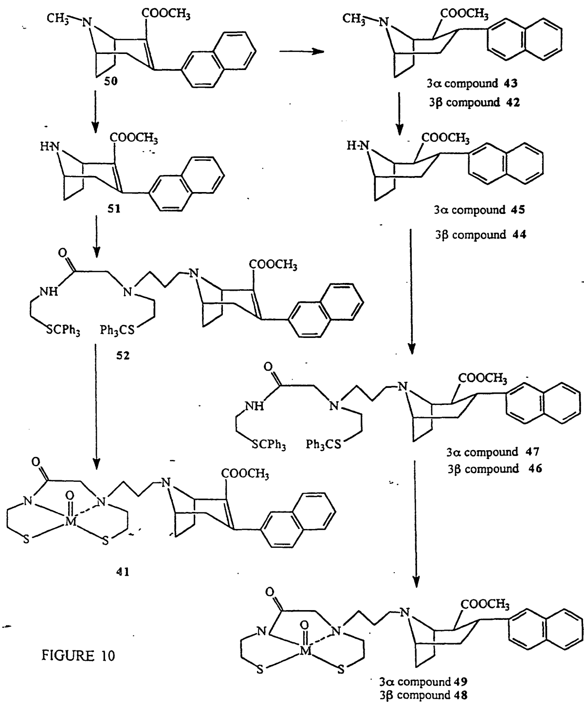
Scheme 9 Synthesis of 3-naphthyl-2-carbomethoxy metal chelates
