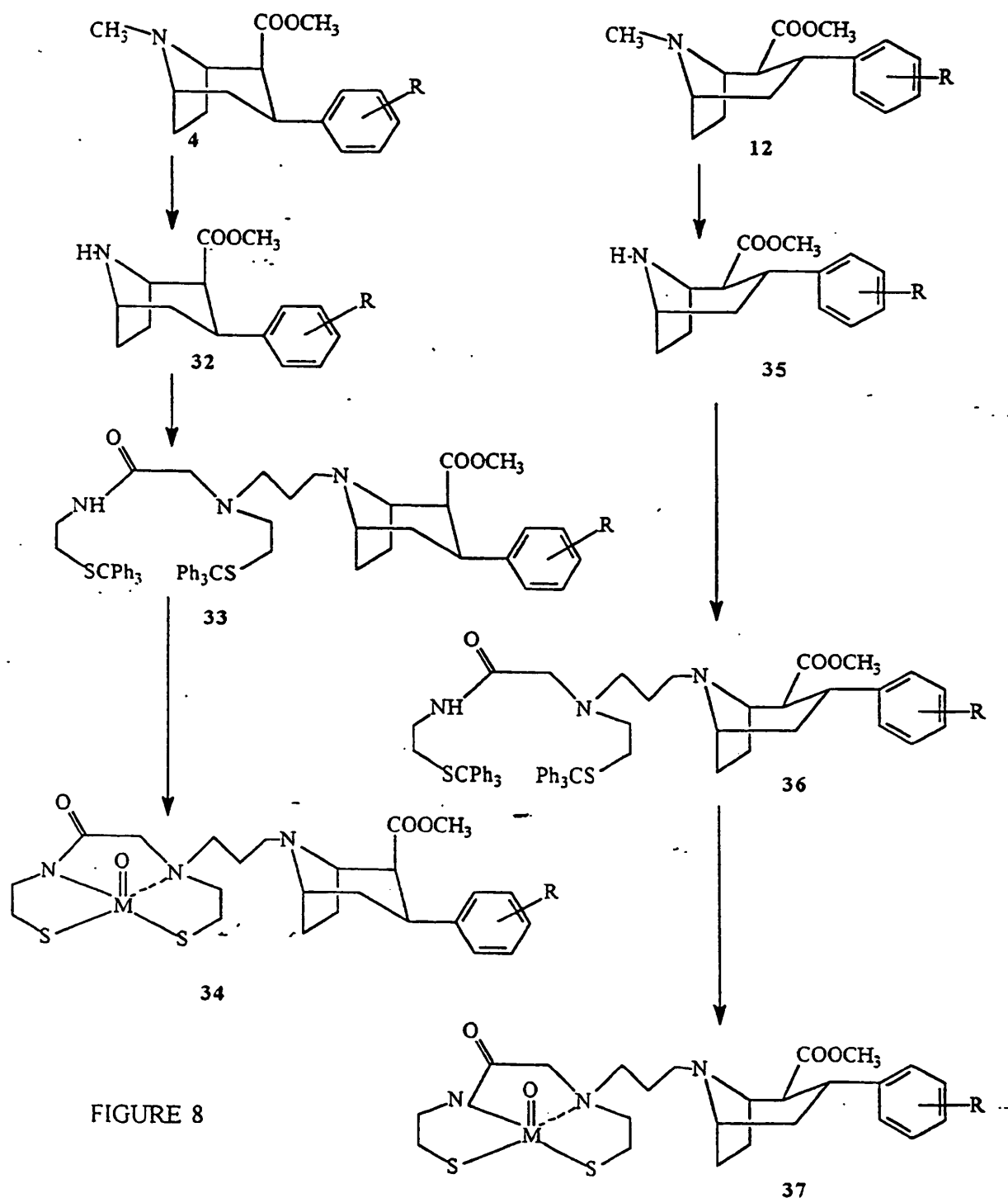
Scheme 7 Synthesis of 3-aryl-2-carbomethoxy metal chelates
