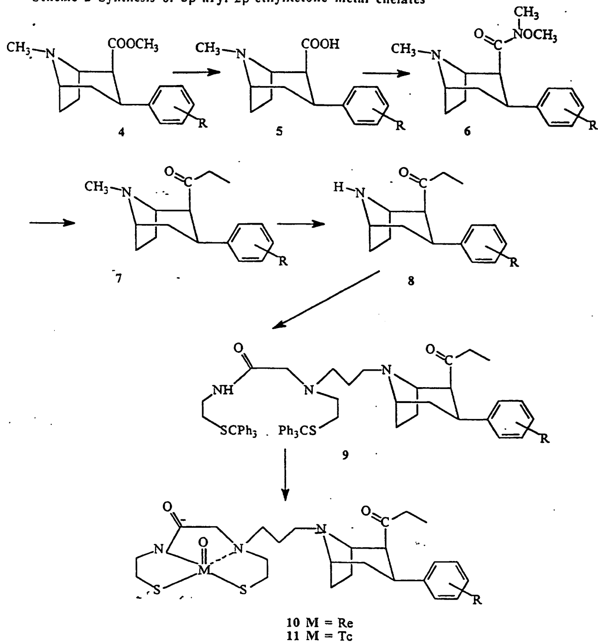
Scheme 2 Synthesis of 3 \beta -aryl-2 \beta -ethylketone metal chelates
