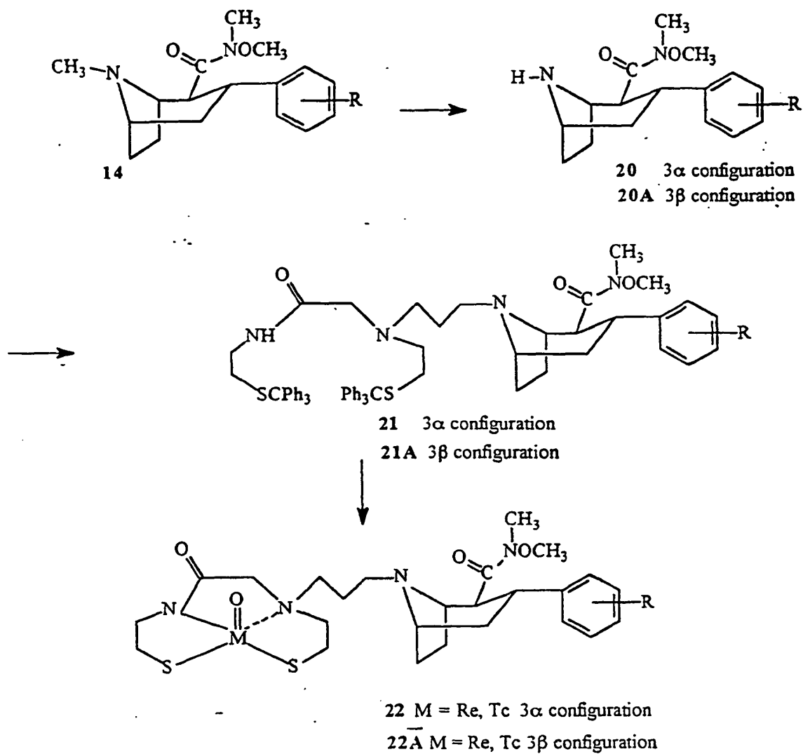
Scheme 4 Synthesis of 2-carboxamido metal chelates
