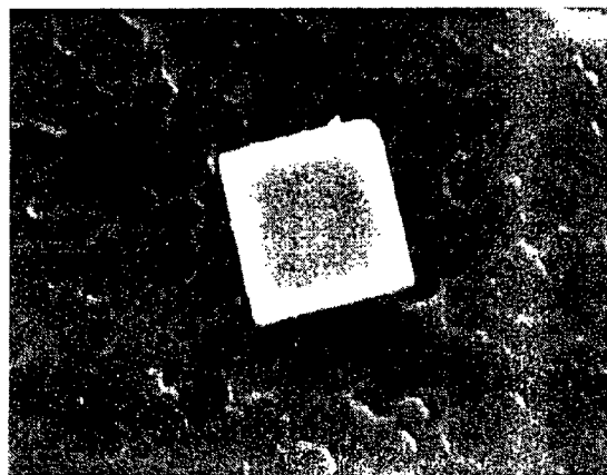
Inclusion ( \text{Ti}(\text{C}, \text{N}) , one side 5\text{ }\mu\text{m} )
