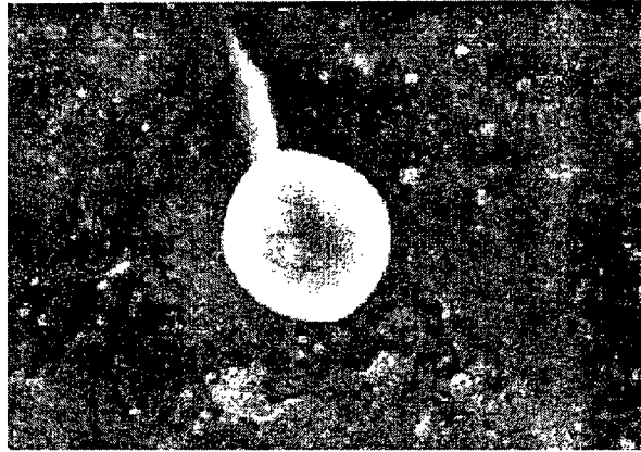
Inclusion ( \text{Al}_2\text{O}_3 , diameter 8\text{ }\mu\text{m} )
