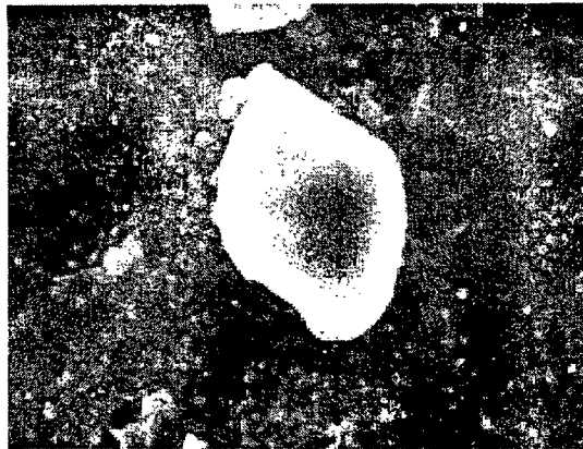
Inclusion ( \text{SiO}_2 , diameter 10\text{ }\mu\text{m} )
