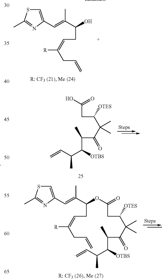
Scheme 5
