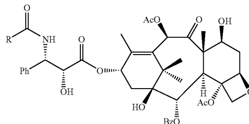
Scheme 1: Taxoids and Epothilones
