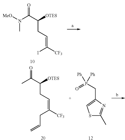
Scheme 3. Synthesis of the alcohol fragment 21
