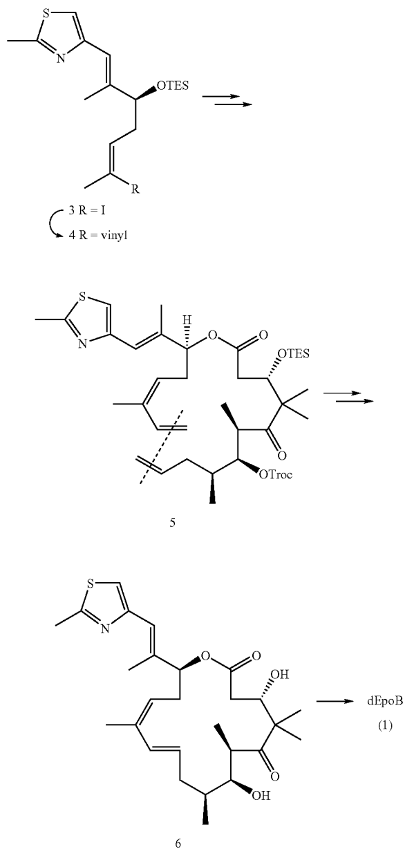
Scheme 1. Synthesis of Epothilone 490
