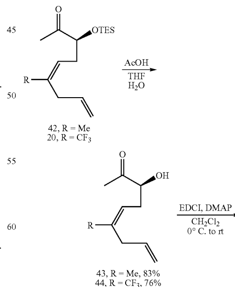
Scheme 8
