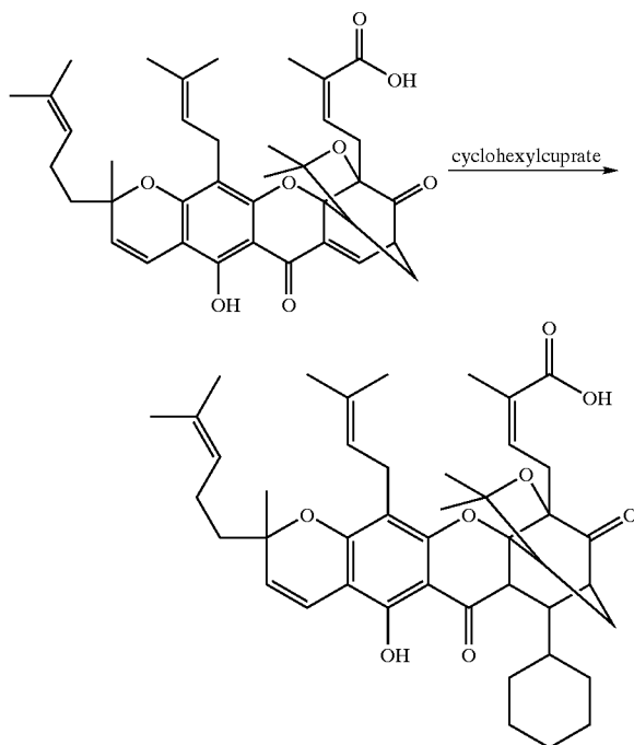
Scheme 10
