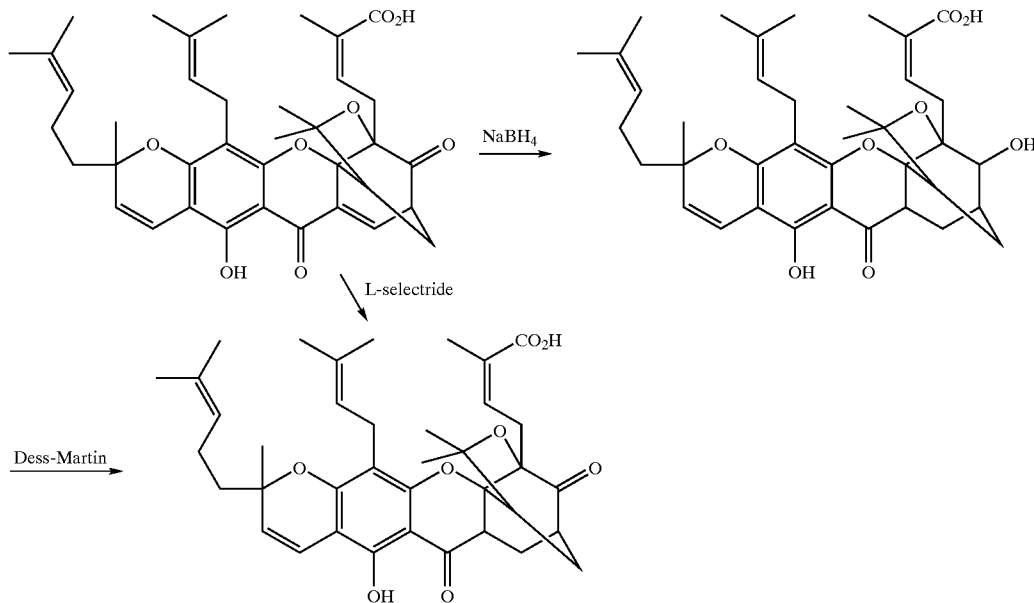
Scheme 9
