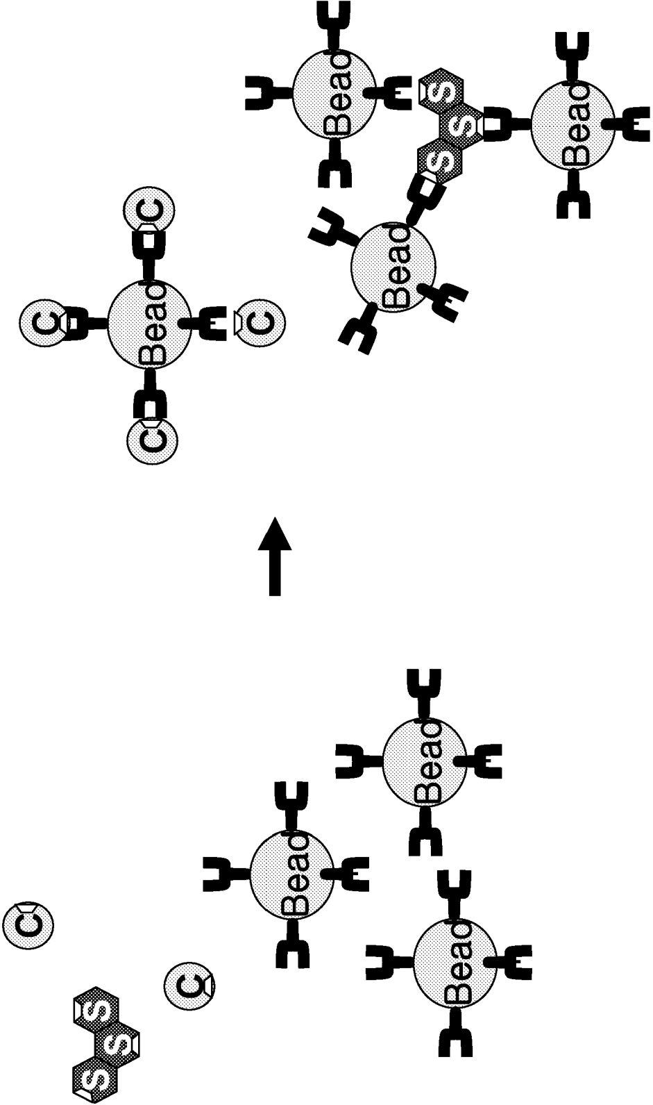
Fig. 2 Agglutination
