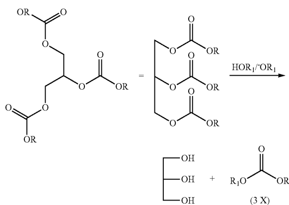
Scheme 1. Illustrative transesterification of tryglycerides with methanol ( \text{HOR}_1 ) with catalytic \text{OH}^- to make biodiesel.
