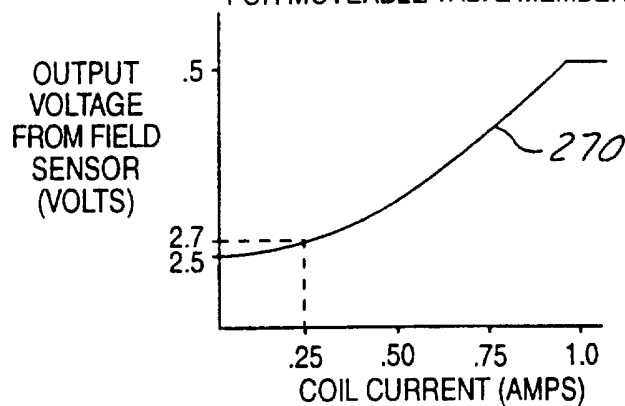
OUTPUT VOLTAGE VERSES COIL CURRENT FOR MOVEABLE VALVE MEMBER
