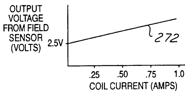
OUTPUT VOLTAGE VERSES COIL CURRENT FOR STATIONARY VALVE MEMBER
