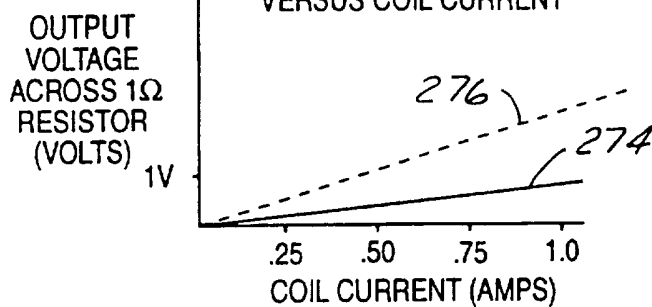
AMPLIFIED FIELD VOLTAGE VERSUS COIL CURRENT
