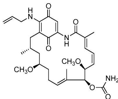
17-(Allylamino)-17-demethoxygeldanamycin
