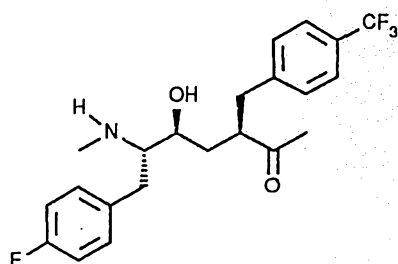
-(p-F)Phe[C](p-CF 3 )Phe-
