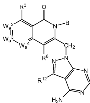
Formula XXIII-B
