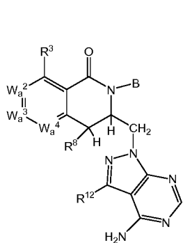
Formula XXIII-A
