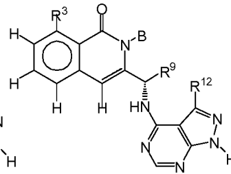
Formula XI-A2
