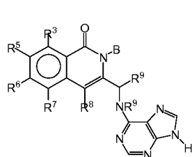
Formula V
