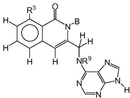
Formula XXVII-C2
