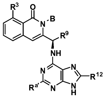
Formula XV-A1
