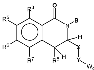
Formula XXVI
