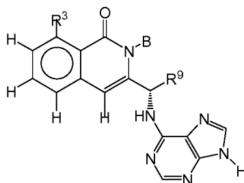
Formula V-A2.
