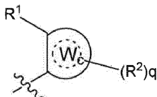
Formel II.
