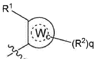
Formel II,
