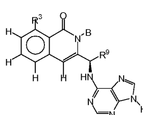
Formula V-A1
