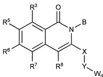
Formula (Ib).
