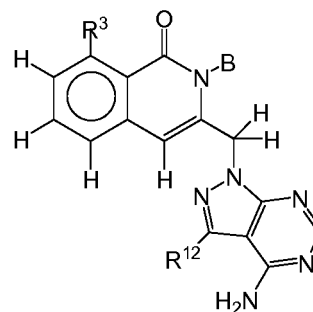
Formula XXVII-A1
