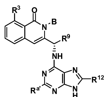
Formula XV-A2
