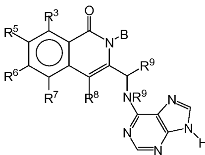
Formula XXVII-C
