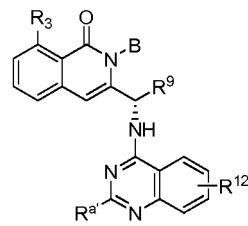
Formula XIX-A3
