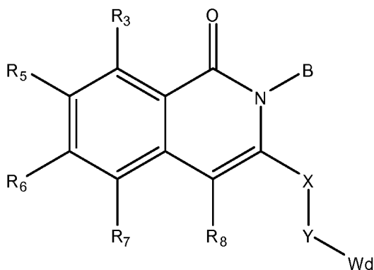
Formula (Ib).
