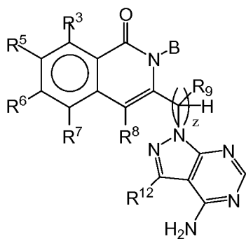
Formula XXVII-B
