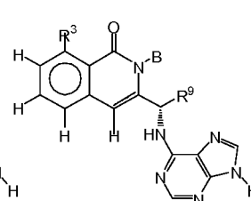
Formula V-A2
