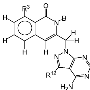
Formula IV-A .
