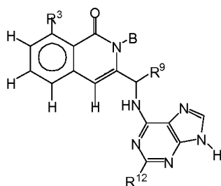
Formula VII-A
