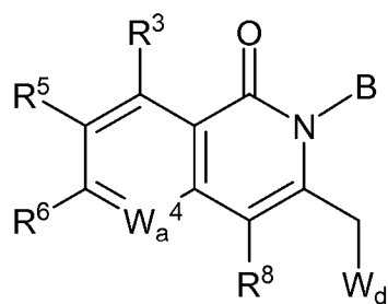
Formula XXVIII
