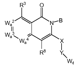
Formula XXIV-B
