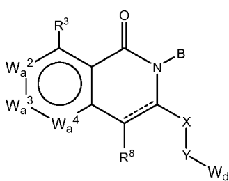
Formula XXV
