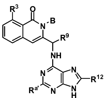
Formula XV-A
