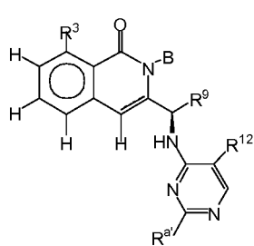
Formula XIV-A1
