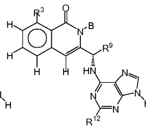
Formula VII-A2
