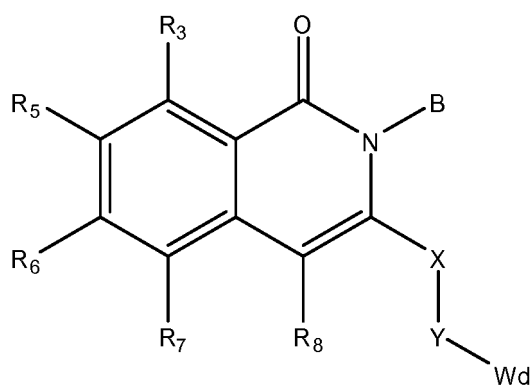
Formula (Ib).
