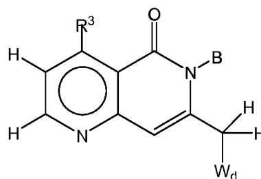
Formula XXVIII-A
