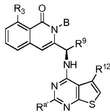
Formula XX-A2
