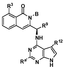
Formula XVI-A1
