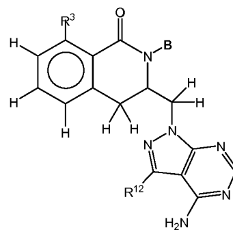
Formula XXVI-A
