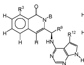
Formula IX-A1
