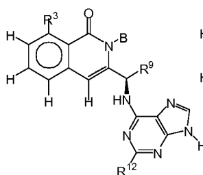
Formula VII-A1
