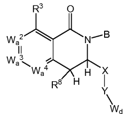
Formula XXIV-A
