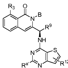
Formula XXI-A2
