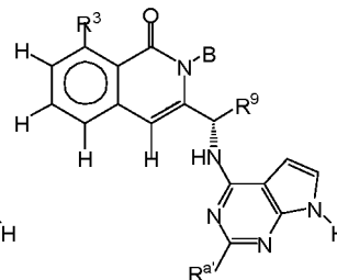
Formula XIII-A2
