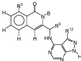
Formula IX-A
