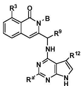
Formula XVI-A
