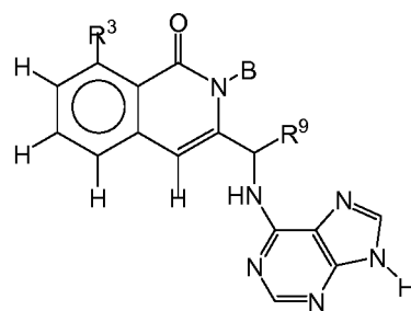
Formula XXVII-C1
