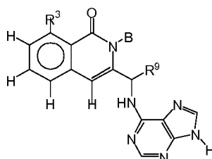
Formula V-A
