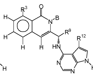
Formula IX-A2
