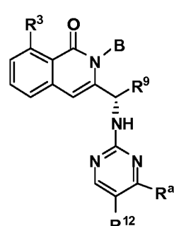
Formula XVIII-A2
