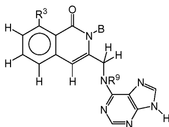
Formula V-B
