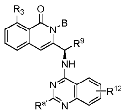
Formula XIX-A2
