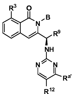
Formula XVIII-A1
