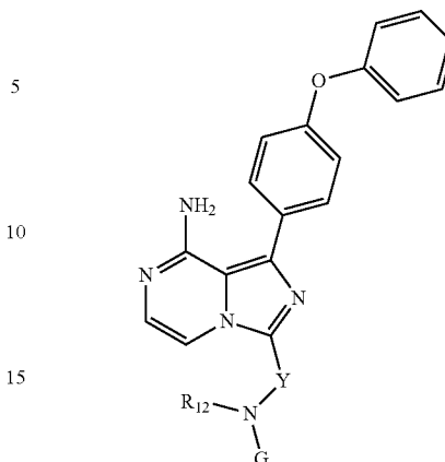
Formula (C2)
