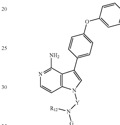
Formula (C3)
