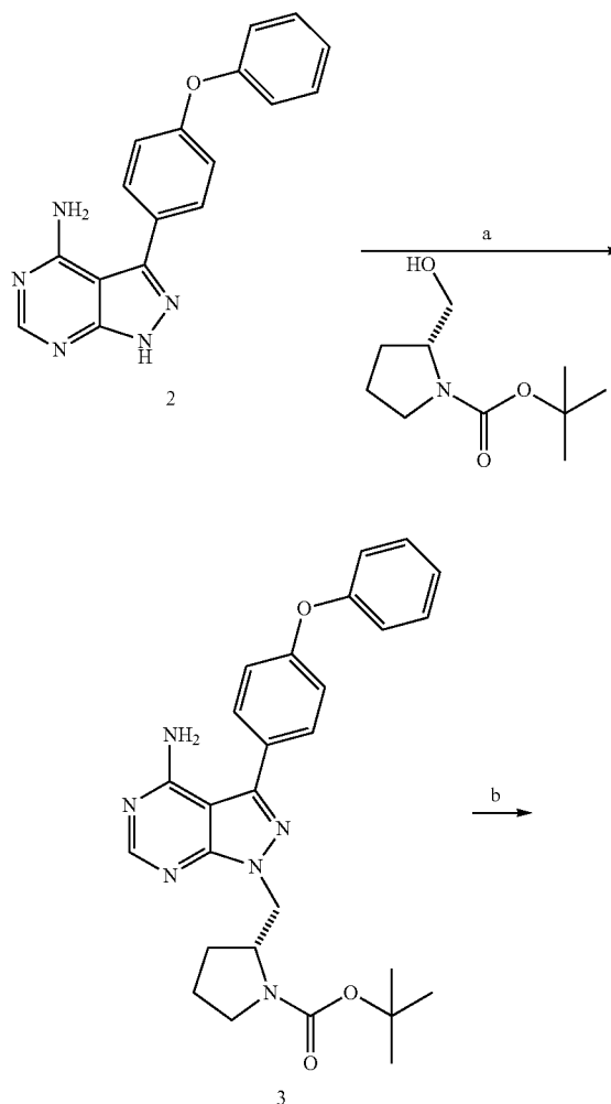
Scheme 1.
