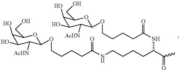
Formula XVI
