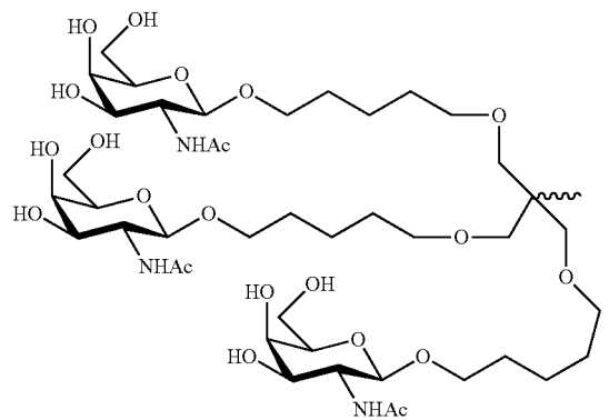
Formula VII
