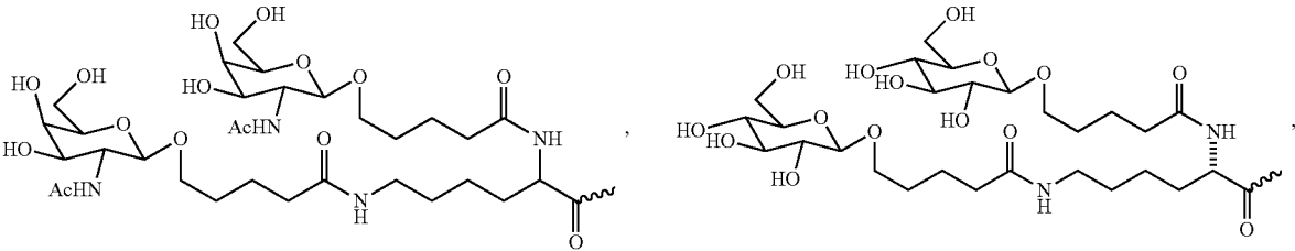
Formula XVI
