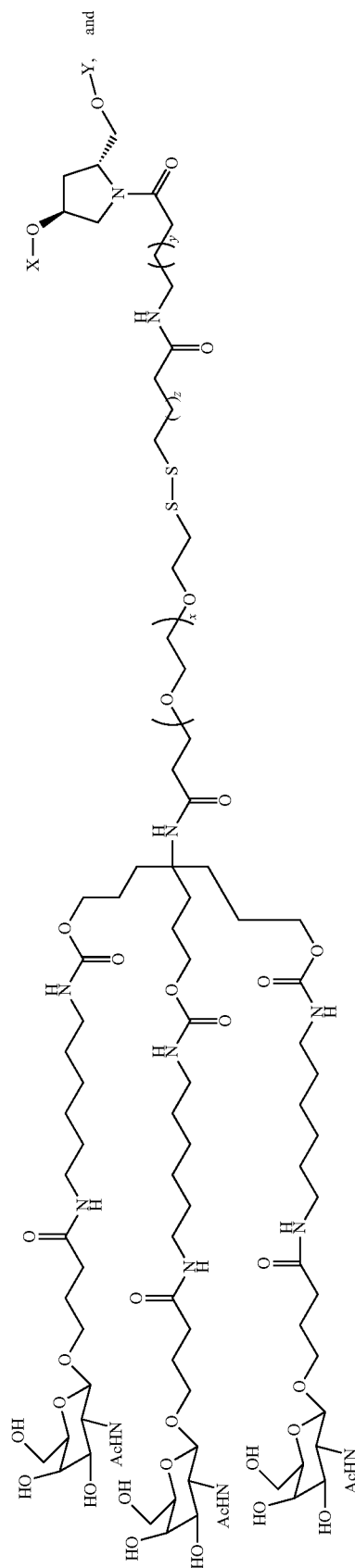
(Formula XXX)
