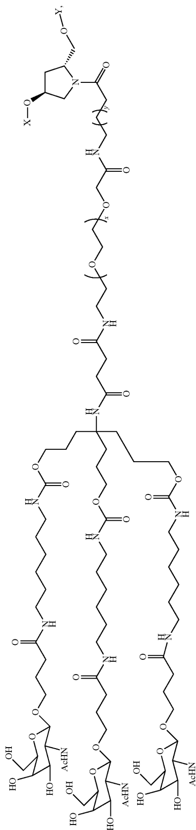
(Formula XXVII)
