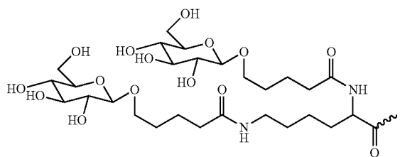
Formula XIX
