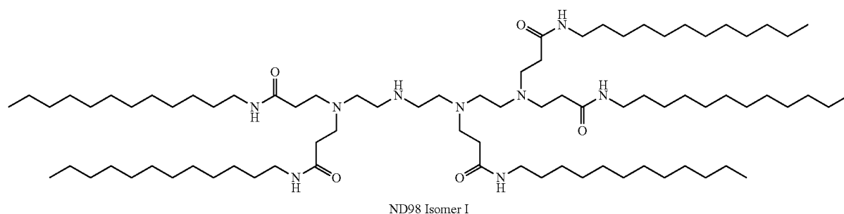
Formula 1
