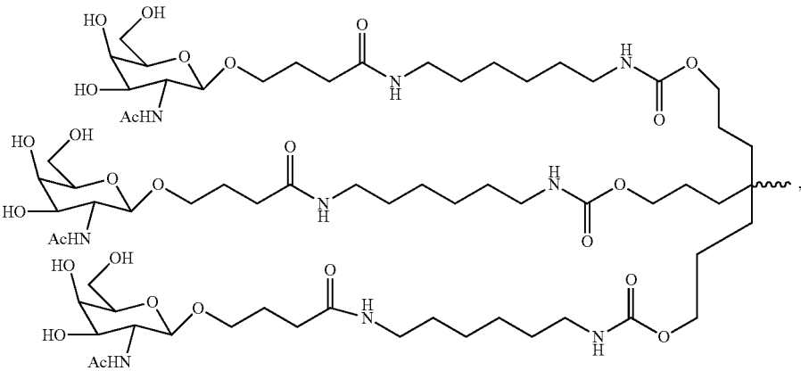
Formula XIV
