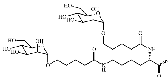
Formula XXI
