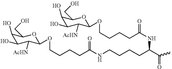
Formula XVII
