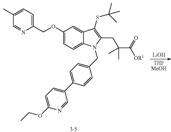
Scheme 4. Hydrolysis and Salt Formation
