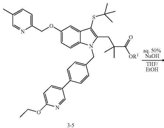
Scheme 5. One-Step Hydrolysis and Salt Formation
