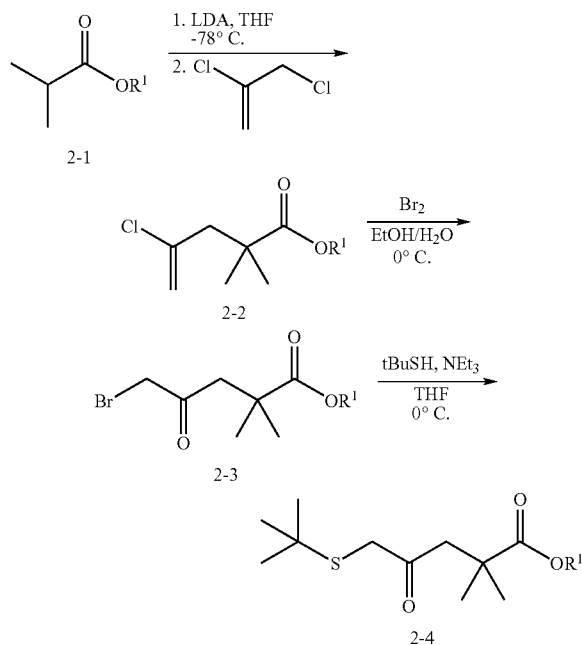
Scheme 2: Preparation of 5-tert-Butylsulfanyl-2,2-dimethyl-4-oxo-pentanoic acid alkyl ester
