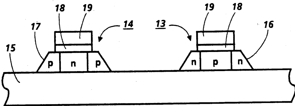
FIG. 2 PRIOR ART
