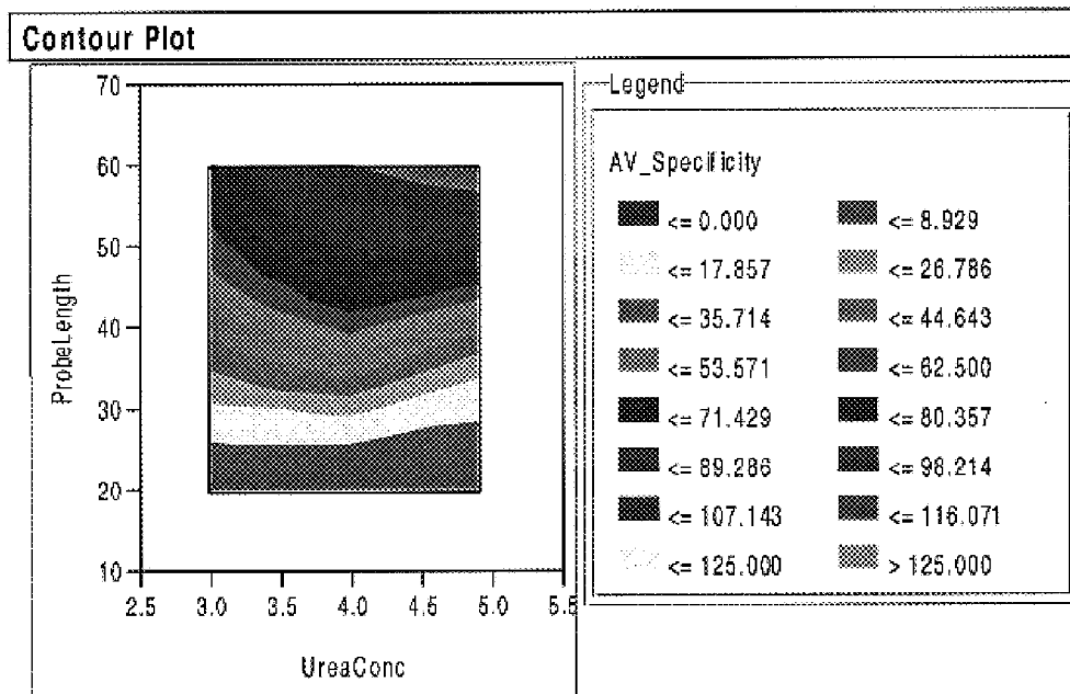
FIG. 5 Extrapolation to Predicted Optimum for L=60 (50°C)
