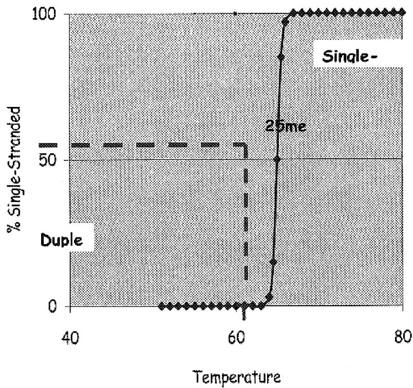
FIG. 3 Duplex Denaturation Curve
