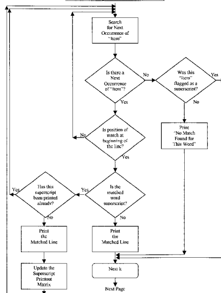
General Flow Diagram of MACRO1 (continued)
