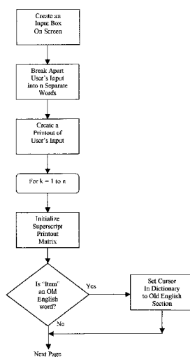
General Flow Diagram of MACRO1
