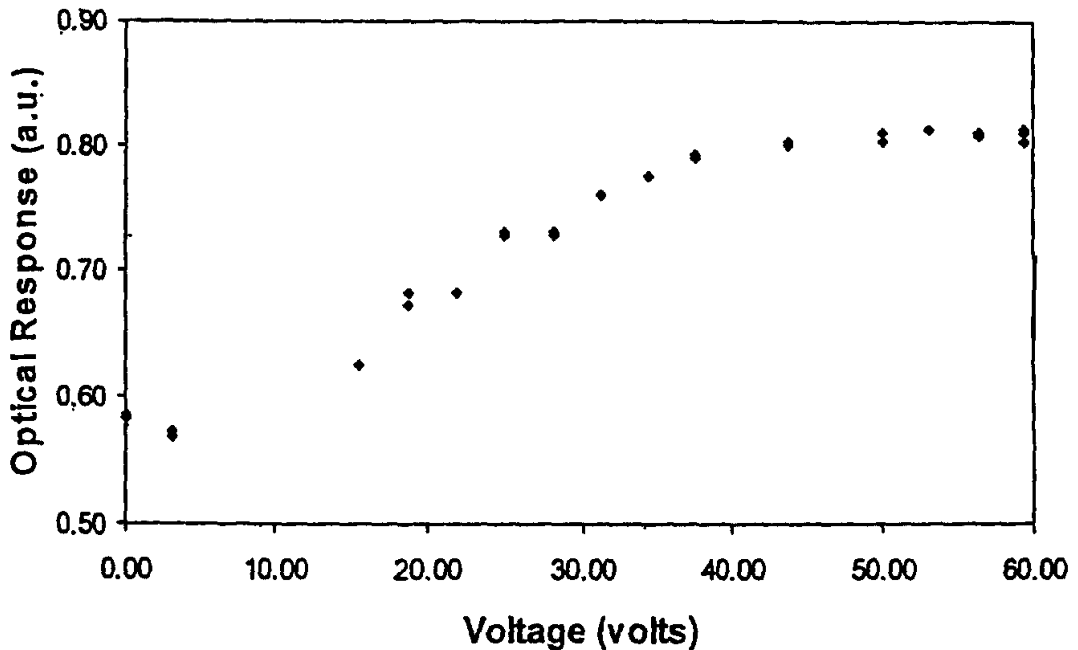
Hysteresis Curve of a LCD of the Current Invention
