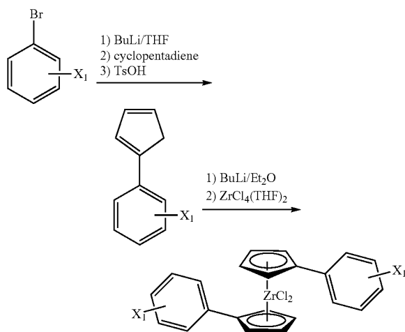
Scheme 1: Generalized Synthetic Scheme for the Preparation of Metallocenes Catalyst Compositions.
