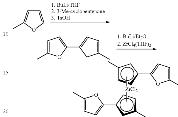
2-Methyl-5-(4-methyl-1,4-cyclopentadien-1-yl)furan
