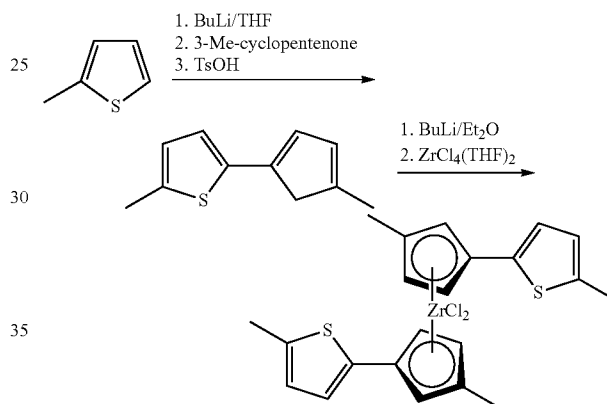
2-Methyl-5-(4-methyl-1,4-cyclopentadien-1-yl)thiophene
