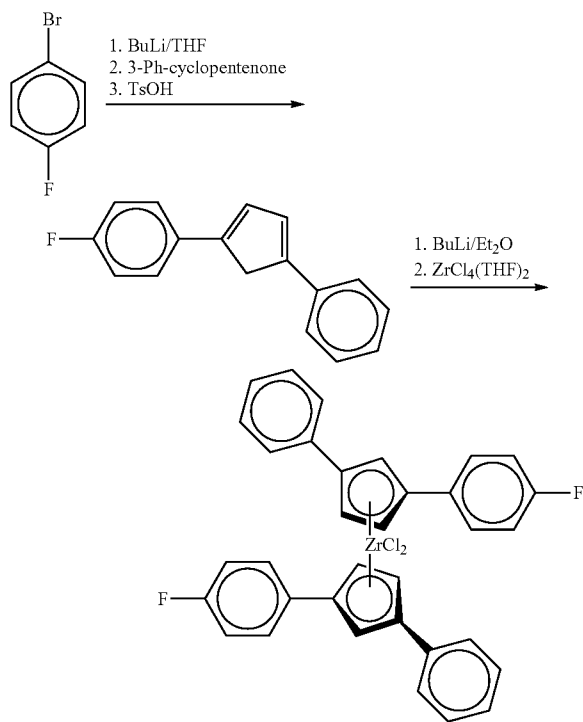
1-Fluoro-4-(4-methyl-1,4-cyclopentadien-1-yl)benzene
