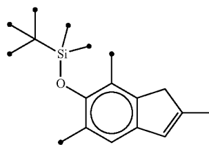
tert-Butyl(dimethyl)[(2,5,7-trimethyl-1H-inden-6-yl)oxy]silane
