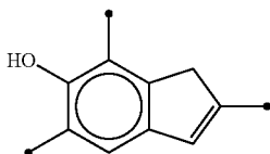
2,5,7-Trimethyl-1H-inden-6-ol
