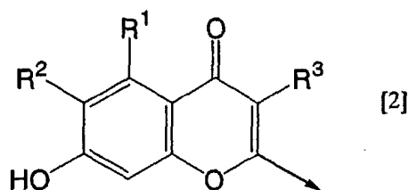
[Chemical formula 18]
