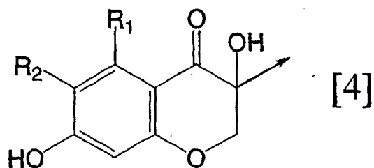
[Chemical formula 5]
