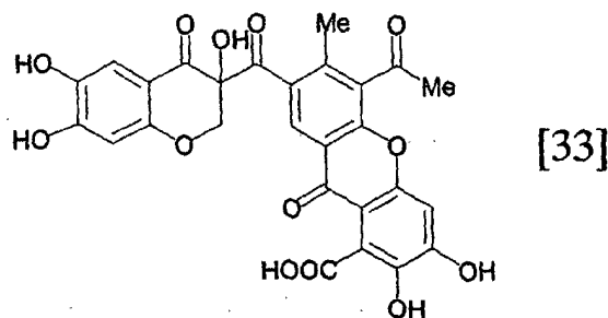
[Chemical formula 48]
