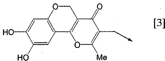
[Chemical formula 4]
