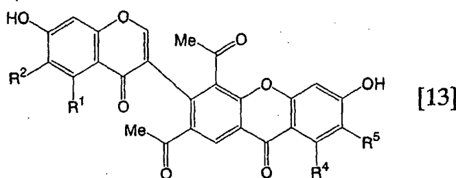
[Chemical formula 26]
