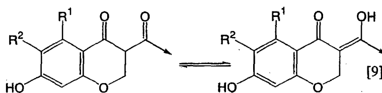
[Chemical formula 20]
