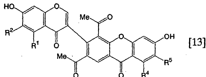
[Chemical formula 27]
