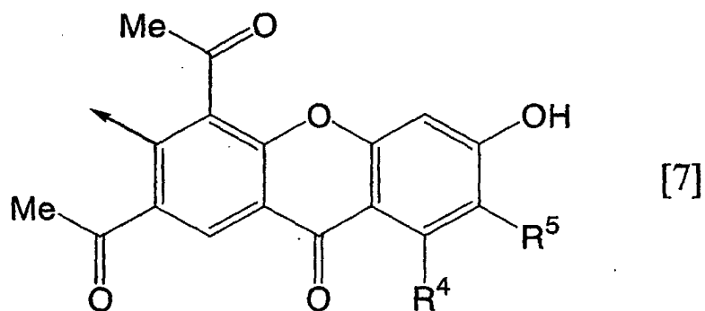
[Chemical formula 16]
