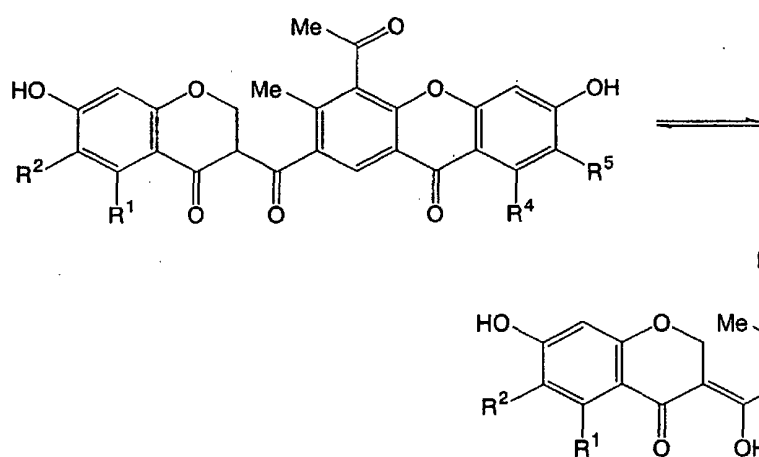
[Chemical formula 24]
