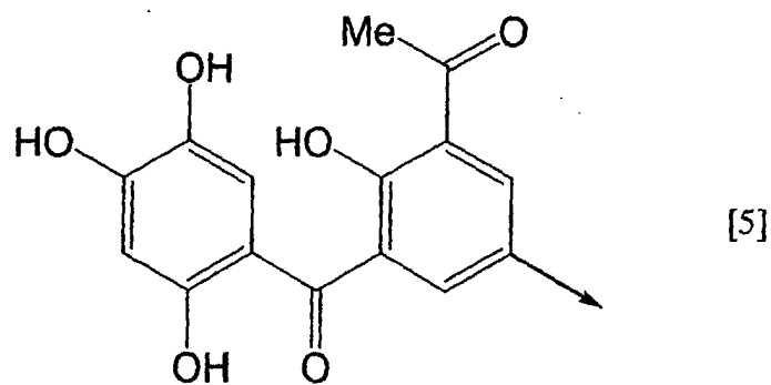
[Chemical formula 14]
