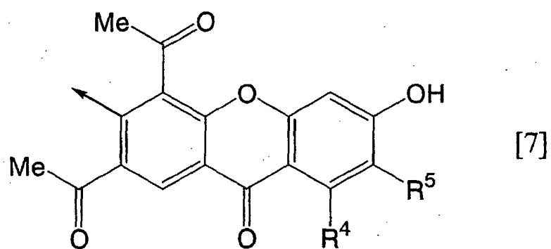
[Chemical formula 8]
