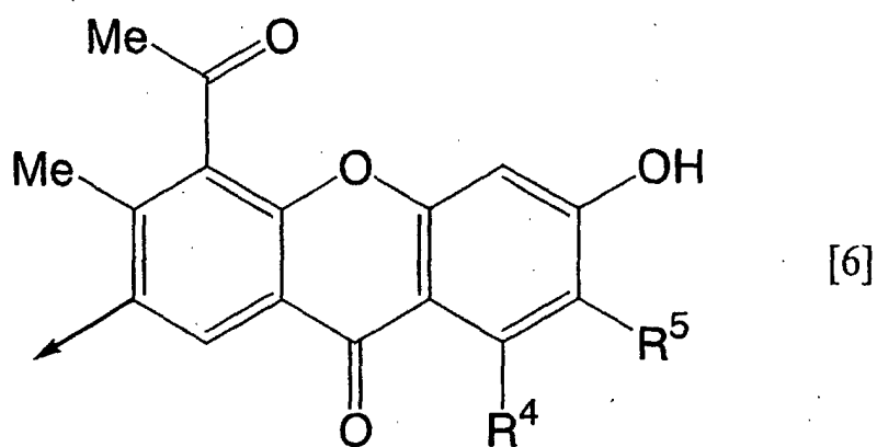
[Chemical formula 7]
