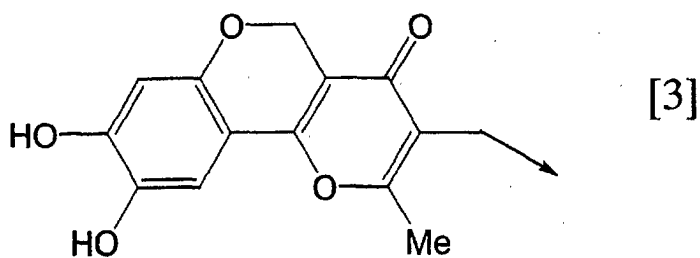
[Chemical formula 12]
