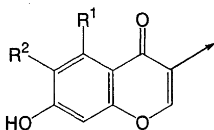
[Chemical formula 23]
