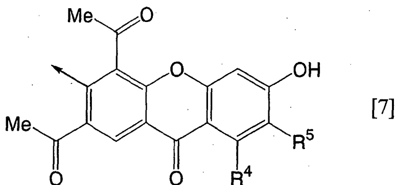
[Chemical formula 16]
