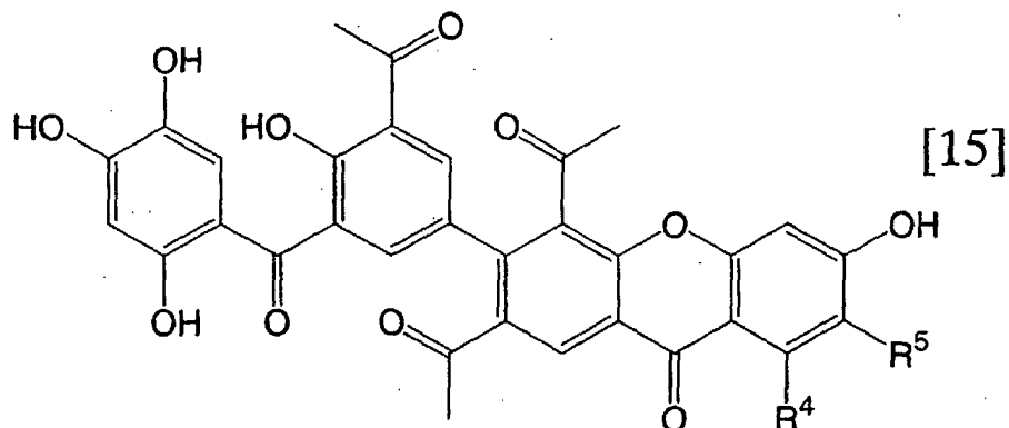
[Chemical formula 30]
