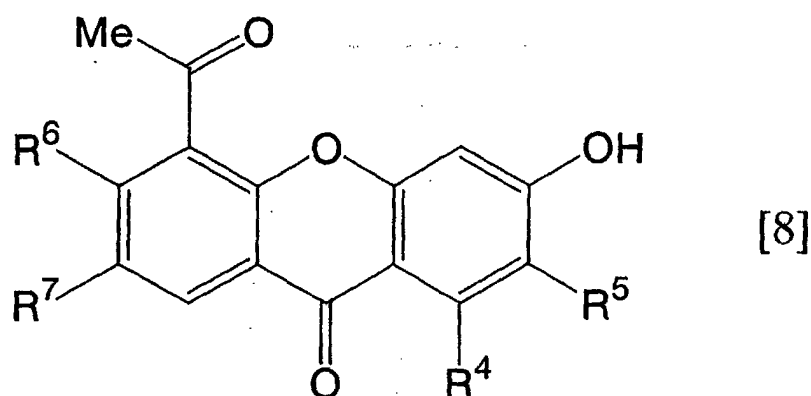
[Chemical formula 17]
