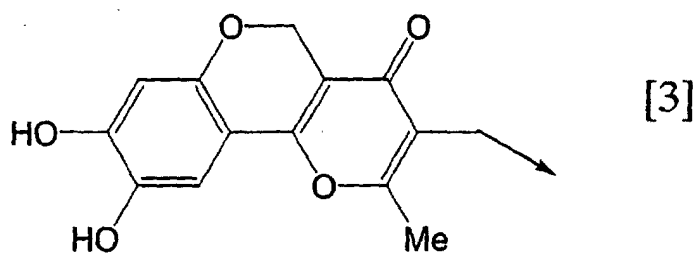
[Chemical formula 19]
