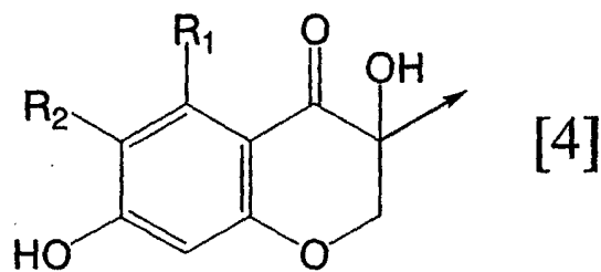
[Chemical formula 5]
