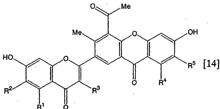
[Chemical formula 28]
