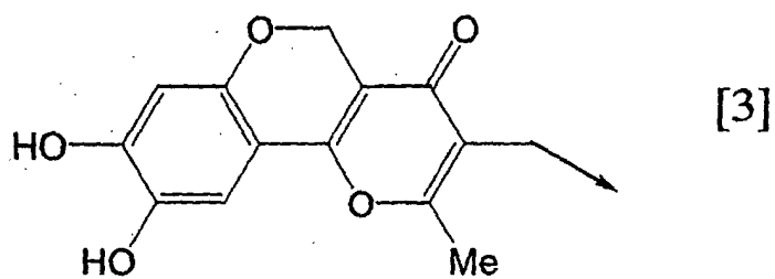
[Chemical formula 12]
