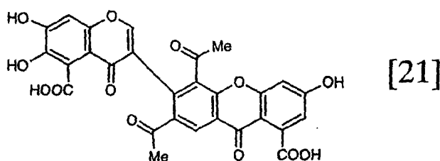
[Chemical formula 36]
