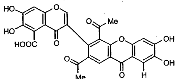
[Chemical formula 33]
