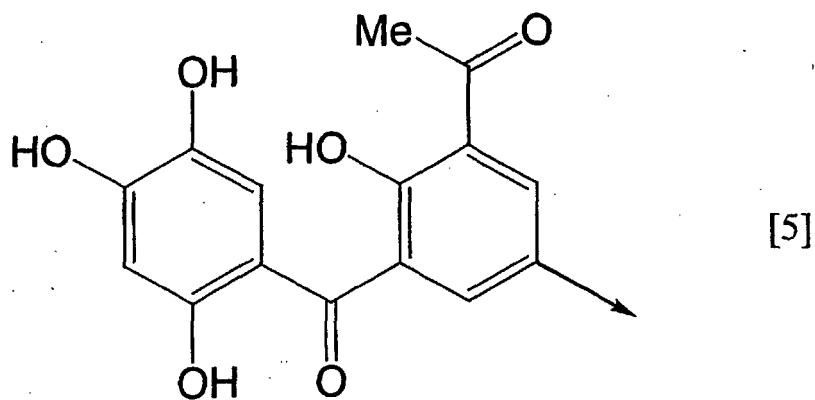
[Chemical formula 14]
