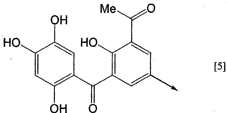
[Chemical formula 22]
