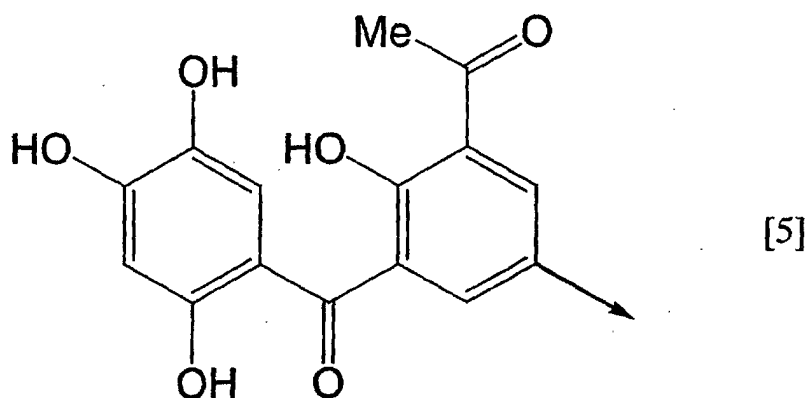
[Chemical formula 6]
