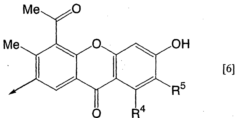
[Chemical formula 15]
