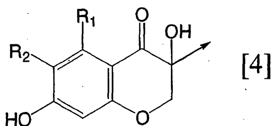
[Chemical formula 13]
