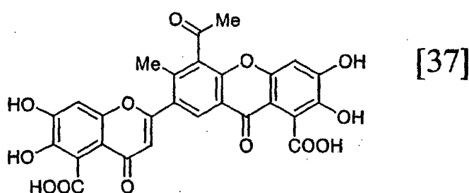
[Chemical formula 52]
