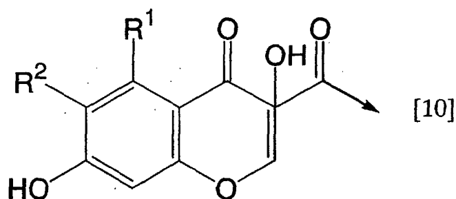
[Chemical formula 21]
