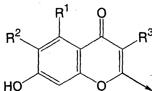
[Chemical formula 3]
