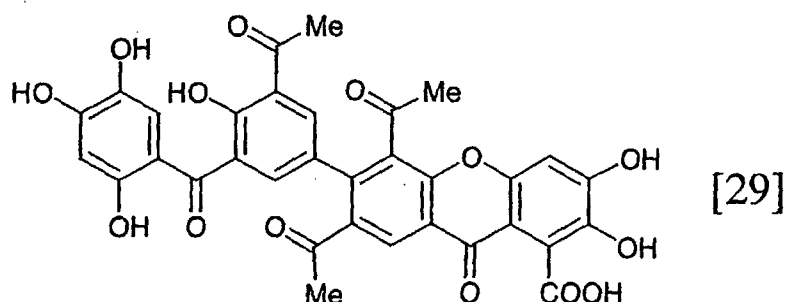
[Chemical formula 44]
