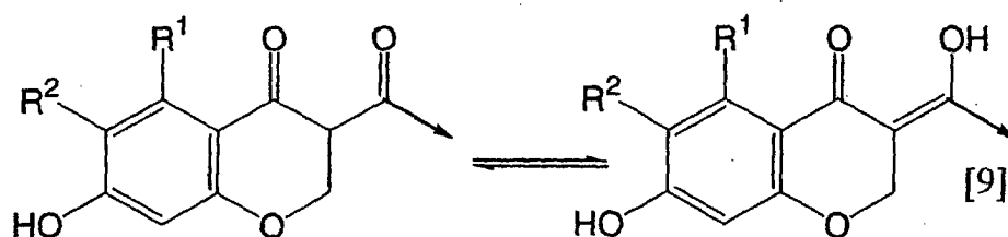
[Chemical formula 20]
