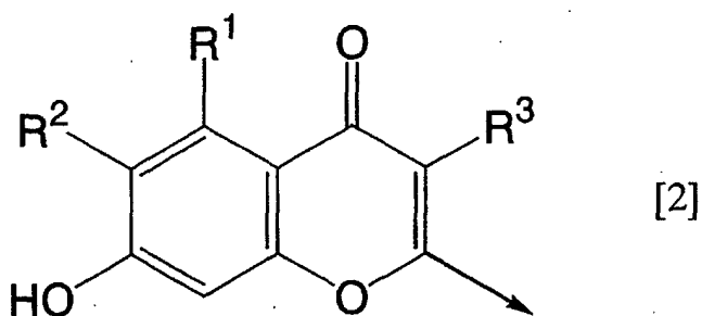
[Chemical formula 11]
