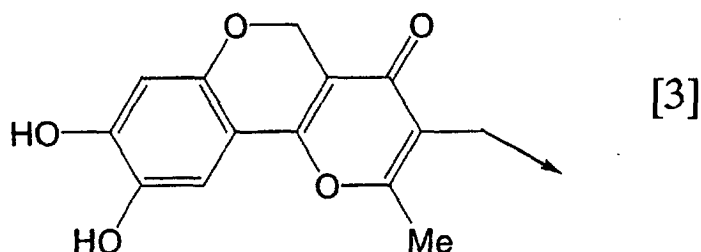
[Chemical formula 29]
