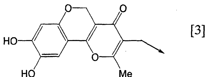
[Chemical formula 19]
