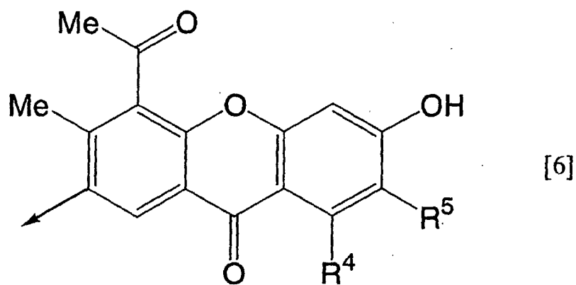
[Chemical formula 7]
