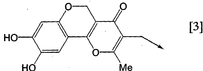
[Chemical formula 29]
