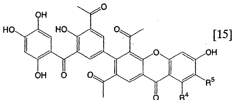
[Chemical formula 30]
