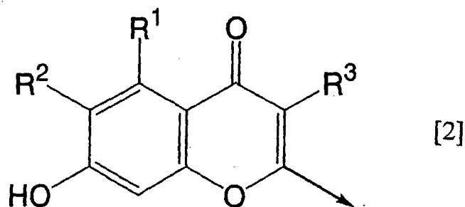
[Chemical formula 3]
