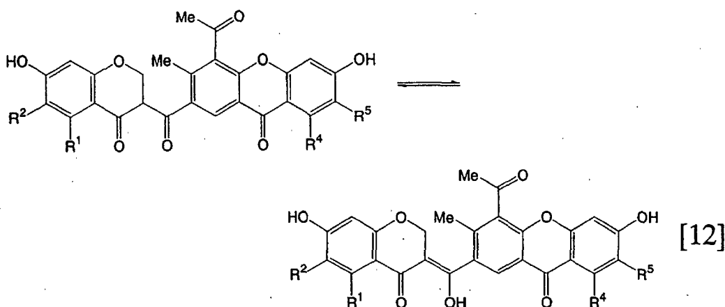
[Chemical formula 25]
