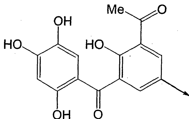
[Chemical formula 22]
