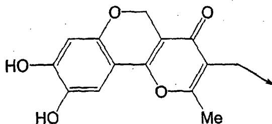
[Chemical formula 4]
