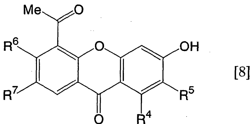
[Chemical formula 17]
