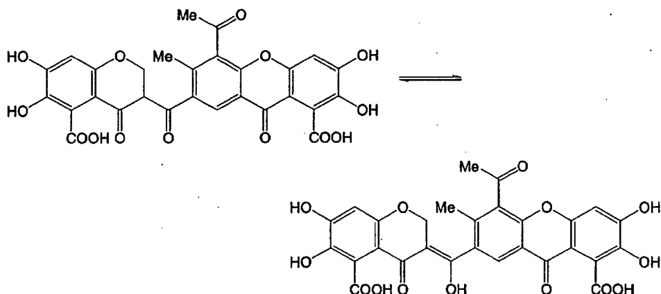
[Chemical formula 32]
