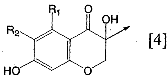
[Chemical formula 13]
