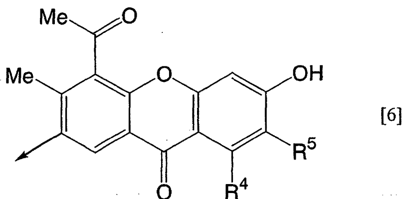
[Chemical formula 15]
