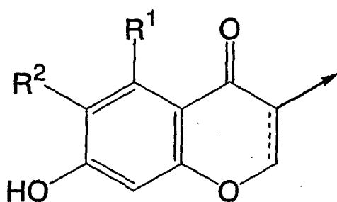
[Chemical formula 1]
