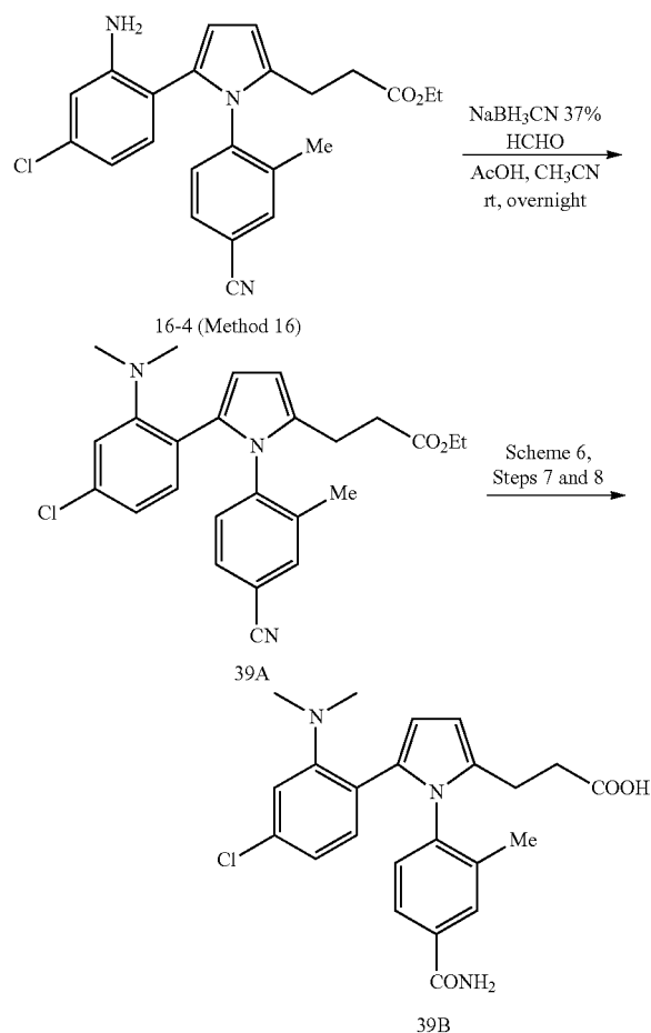
Scheme 39: Synthesis of 3-(1-(4-carbamoyl-2-methylphenyl)-5-(4-chloro-2-(dimethylamino)phenyl)-1H-pyrrol-2-yl)propanoic acid
