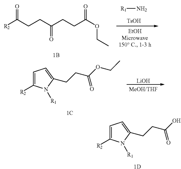
Scheme 1A: Alternate conditions
