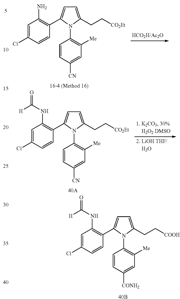
Scheme 40: Synthesis of 3-(1-(4-carbamoyl-2-methylphenyl)-5-(4-chloro-2-formamidophenyl)-1H-pyrrol-2-yl)propanoic acid
