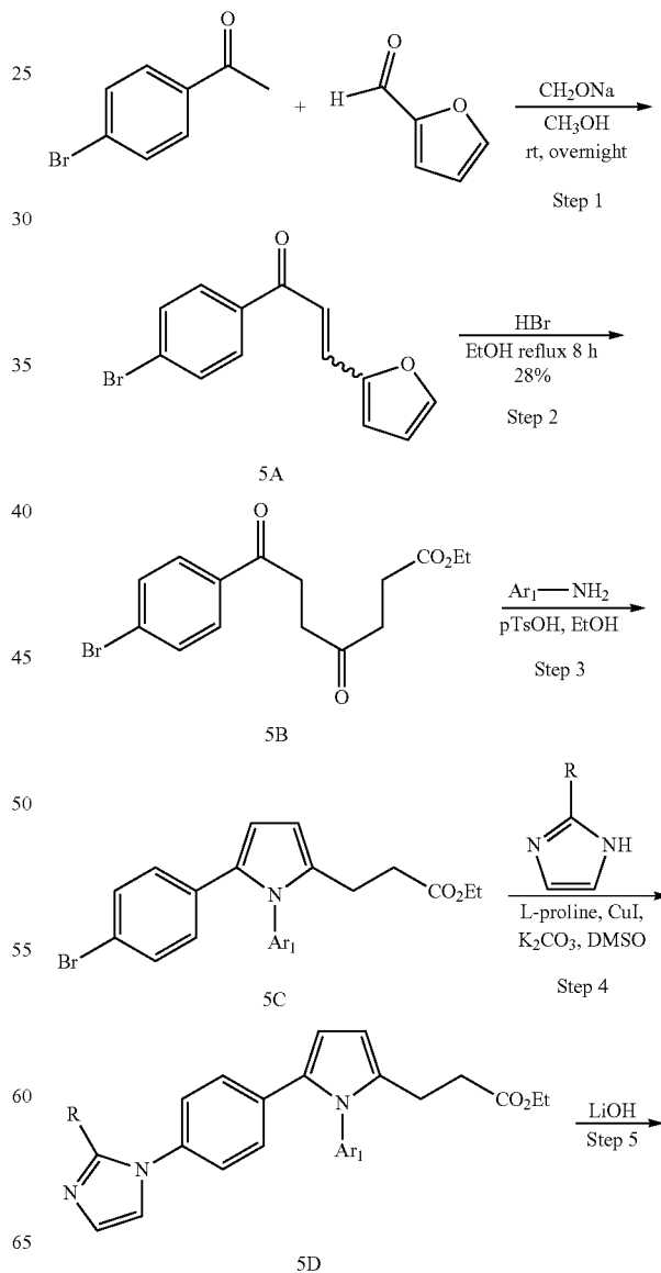
Scheme 5: A general scheme for preparing GSNOR inhibitors with structure 5E
