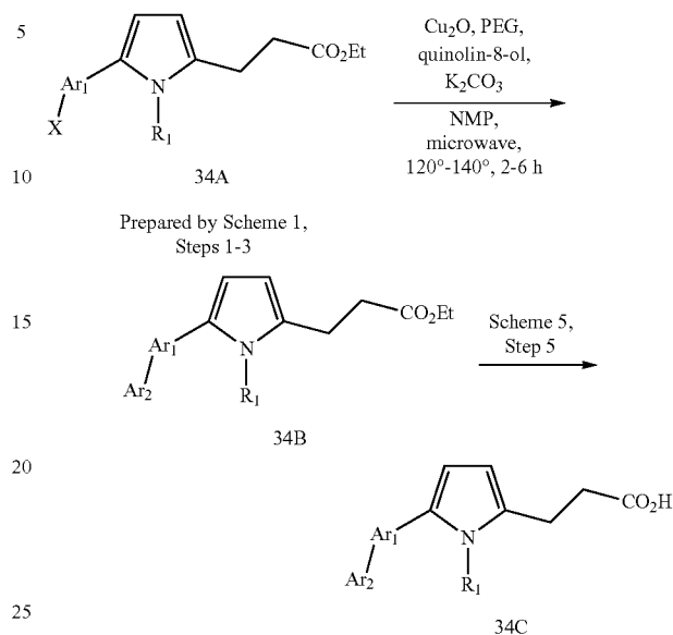
Scheme 34: general scheme for preparing GSNOR inhibitors with structure 34C
