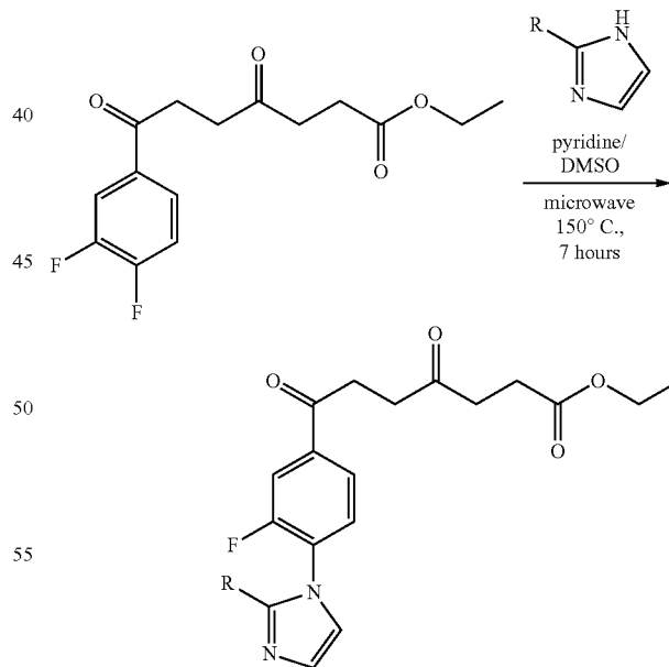
Scheme 36A: Alternative conditions for making Compound 36B-type intermediates (Scheme 36 above).
