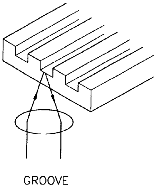
FIG. 3C (PRIOR ART)
